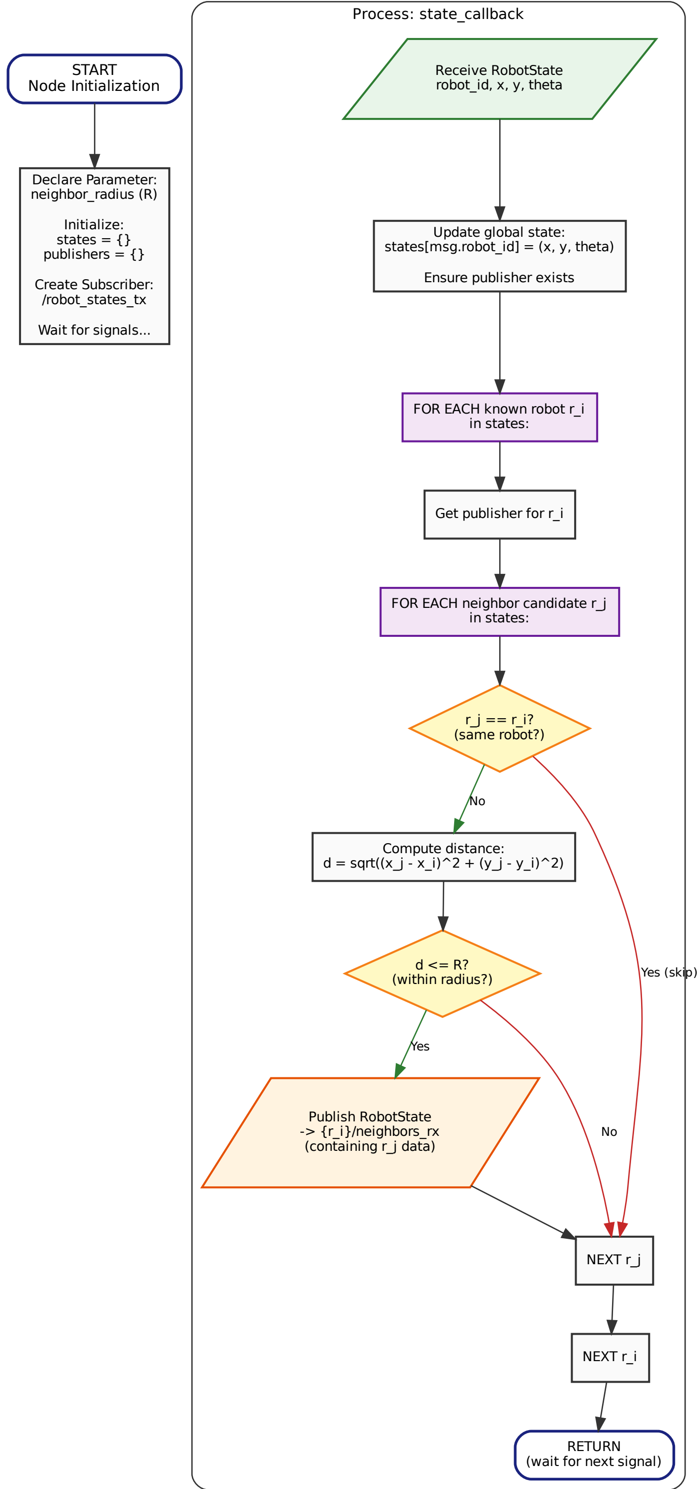
Process SDL Diagram - AIRE Node (Neighbor Router)
