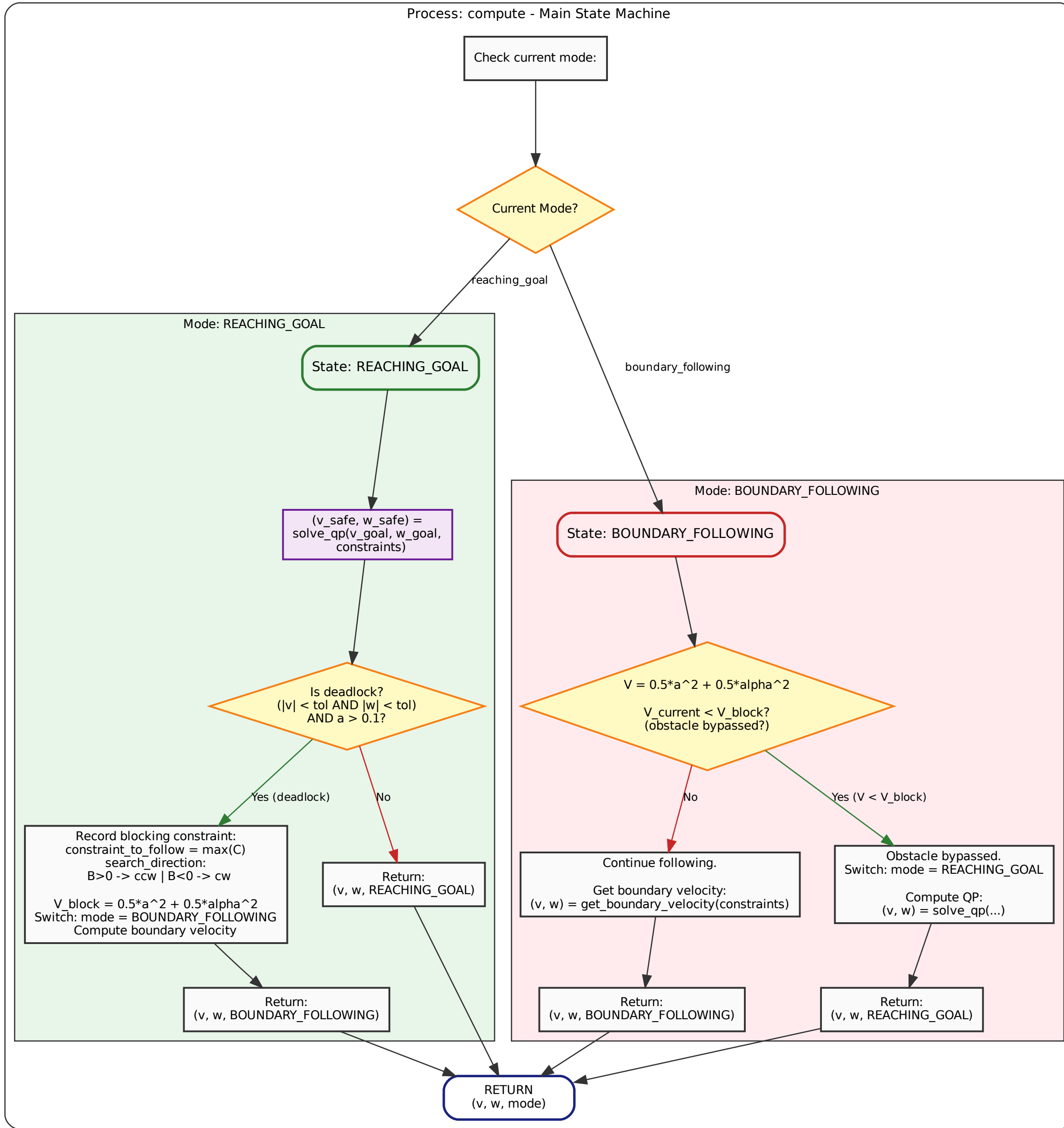
Process SDL Diagram - PVA Algorithm (State Machine)
