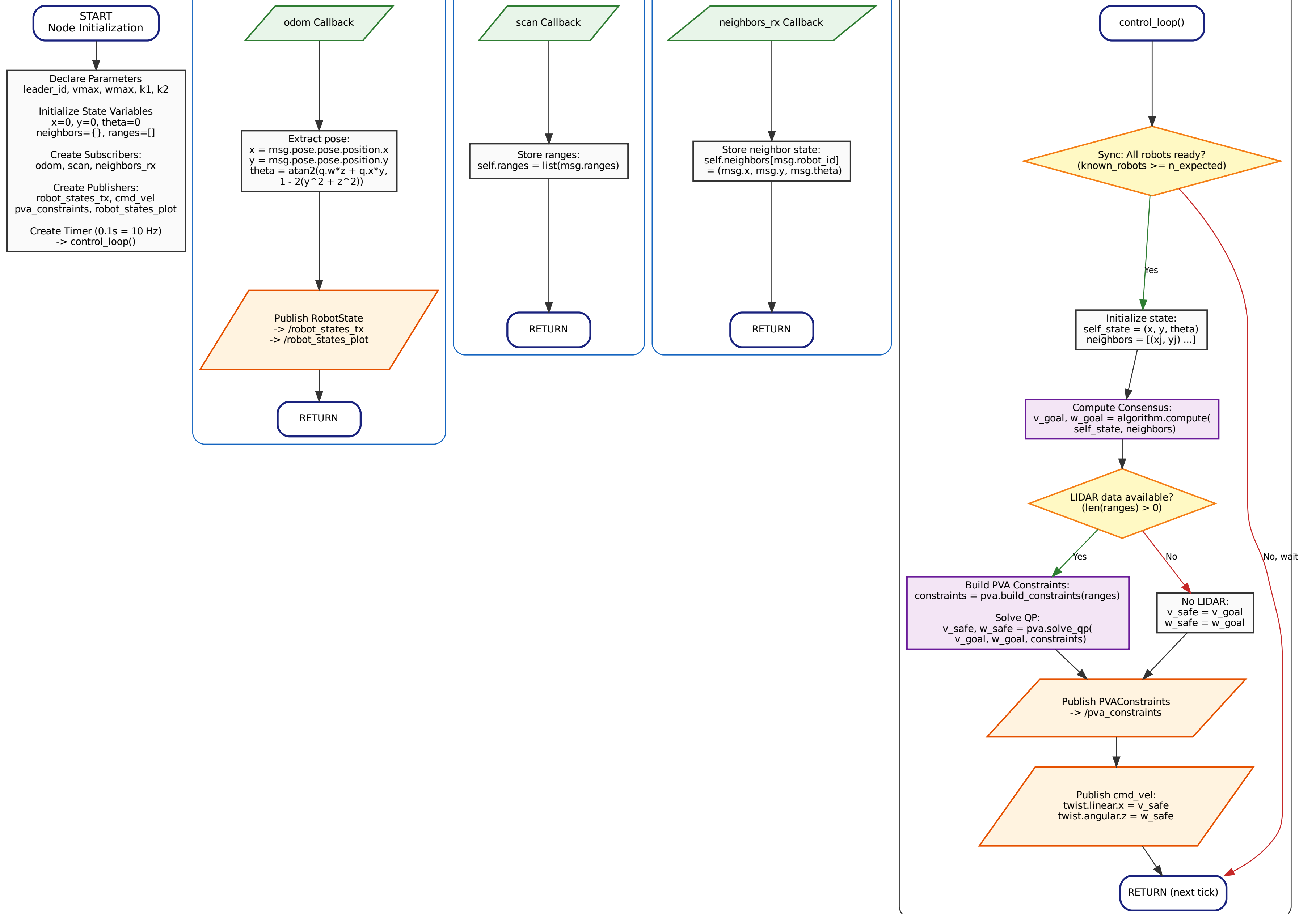
Process SDL Diagram - Robot Control Node
