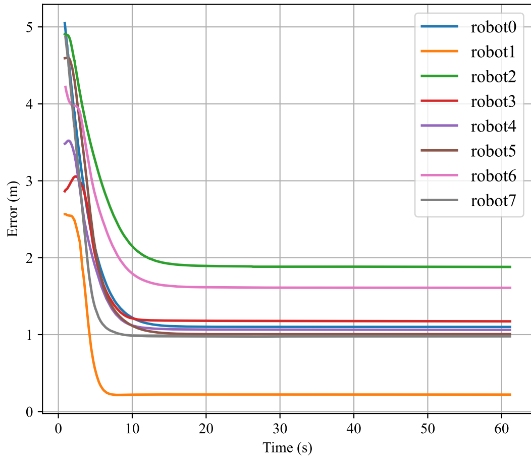
Formation error evolution
