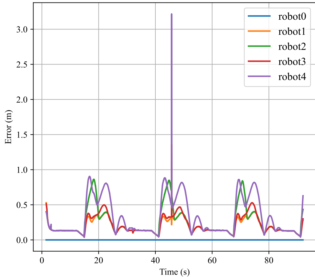
Formation error evolution
