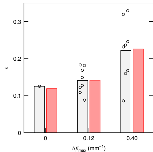
Figure 5 | Averaging over different noise realizations. Experimentally measured transfer efficiency in photonic maze structures with the topology of Fig. 3 and propagation length t=60 mm. Both uniform and different noise maps with \Delta\beta_{\max}=0.12\text{ mm}^{-1} and \Delta\beta_{\max}=0.40\text{ mm}^{-1} have been implemented. The light grey (left) bars indicate the average over several experimental results obtained for different noise maps with the same amplitude \Delta\beta_{\max} (single measurements are reported as open circles). The red (right) bars represent the expected average transfer efficiency, numerically simulated for 1,000 different noise maps with the given \Delta\beta_{\max} . Error bars are smaller than the mark size.
