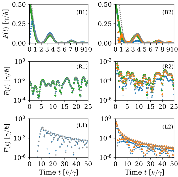
FIG. 1: Comparison of F^\Psi(t) (gray squares), F^\Phi(t) (blue +), the Zeno approximation [green \circ , Eq. (68), not for (L)], and the corrected non-Hermitian approach with an additional factor four (orange \triangle , only right column). For the benzene ring (B), the random Hamiltonian (R) and on the infinite line (L). Detection is performed at the origin |\psi_d\rangle = |0\rangle . Detection period is given by \tau = 0.5\hbar/\gamma (B,L) or \tau = 0.25\hbar/\gamma (R). Initial states are |\psi_{\text{in},1}^{B,R}\rangle and |\psi_{\text{in}}^L\rangle = |20\rangle for the left column (1) and |\psi_d\rangle for the right column (2). For the benzene ring the data was interpolated between the times n\tau to better compare the area t \approx \tau . In the transition problem F^\Psi(t) , F^\Phi(t) and the Zeno approximation agree almost perfectly for t \gtrsim \tau , but differ for small times (see B). In the return problem a factor four must be introduced to F^\Psi(t) to match the stroboscopic data (orange triangles). This also holds for the complicated dynamics of the random Hamiltonian.
