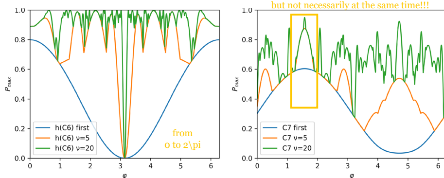
Fig. 6 Plot of phase-dependent transport performance for h(C6) (left) and C7 (right). For each graph we compare the result obtained using first maxima with what is obtained with maximization with bounds set up with different values of \nu . As for time performance the plot for each value of \nu acts as a lower bound for any higher choice of it
