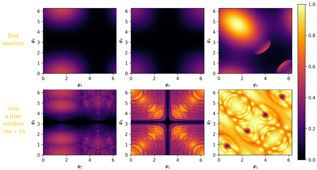
Fig. 8 Transport probability as a function of the two free phases for C9/C4 (left), C8+C8 (centre) and DiC4 (right) (c, f). The upper row show transport events corresponding to first maxima, whereas the lower row show results obtained by optimization over a linear time window with \nu = 10
