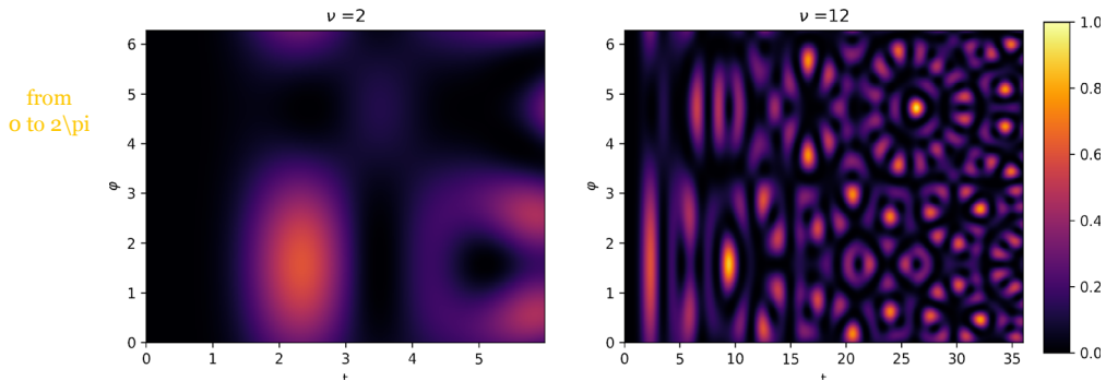
Fig. 3 Evolution of localization probability on target site for C7 as a function of time ( x ) and phase applied to the cycle ( y ). The two plot represent the same evolution on 2 different time window, \nu (see below) is, respectively, set to 2 ( a ) and 12 ( b ). It is evident how difference in applied phase may result in two completely unrelated evolutions
