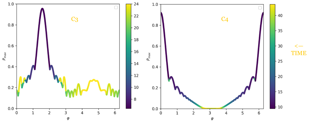
Fig. 9 Transport probability as a function of the single phase parameter , for 10-unit optimal chains (see “Appendix A”), with C3 units (left panel) and C4 units (right panel). Transport maxima are chosen with the linear time window criterion ( \nu is set to 2), transport time is drawn as color map according to the shown colour bars
