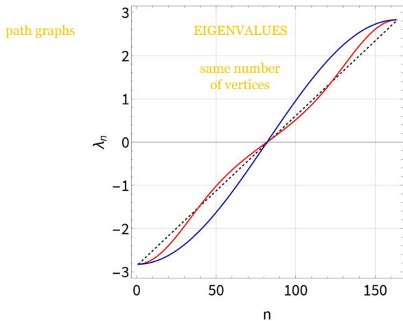
Fig. 15 Spectra of Hamiltonians for path graph (dark blue) with 163 sites and for the C3 chain with handles and optimal phase with 80 triangle units (red) . The total number of vertices is the same for both graphs . n labels the eigenvalues sorted in increasing order. The dotted black line shows the linear trend for reference . Notice that minimal modulation of weights on the path graph will not visibly change the blue curve (Color figure online)
