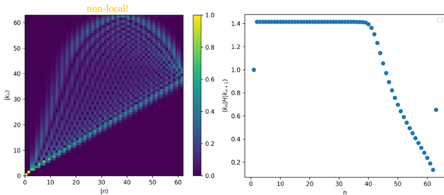
Fig. 13 Modulus of overlap between Krylov basis and site basis states \langle j | k_n \rangle (left) and couplings between the Krylov states \langle k_n | H | k_{n+1} \rangle (right) for a C3 chain of 30 units with optimal phase
