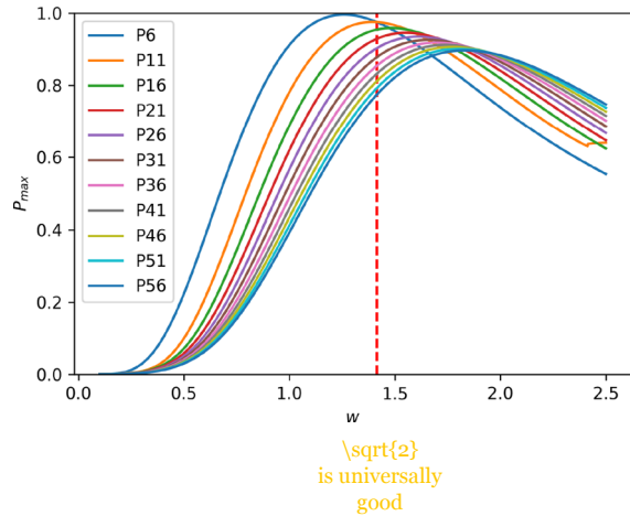
Fig. 14 Transport performance of first maxima as a function of speedup for a sample of P_w graphs. The speedup parameter obtained for C3 and C4 chains ( w = \sqrt{2} ) lies around the optimal value of many P graphs
