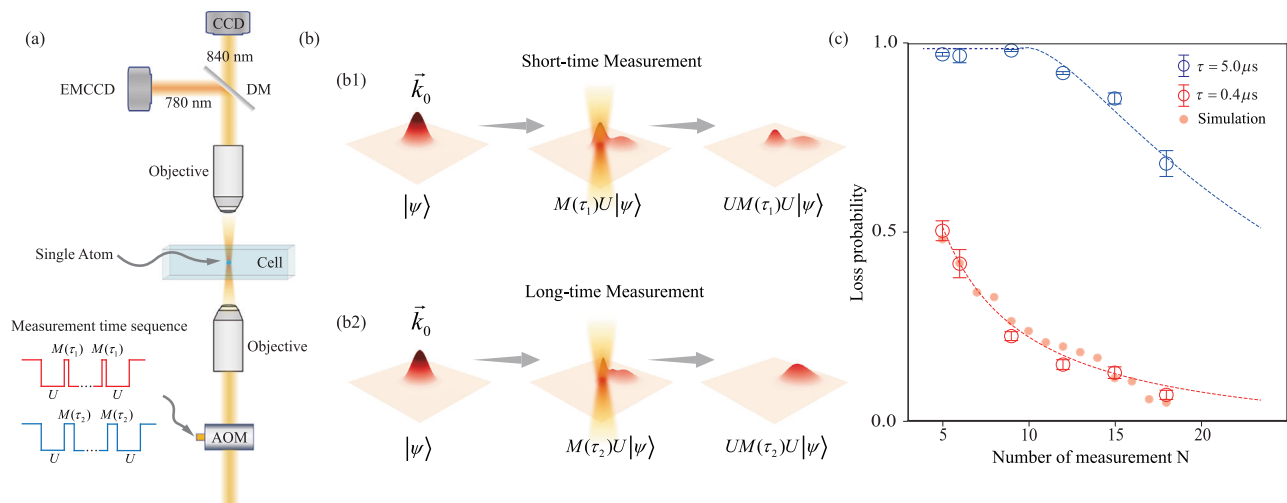
Fig. 1 | Physical diagram and observation of the Quantum Zeno Effect.
