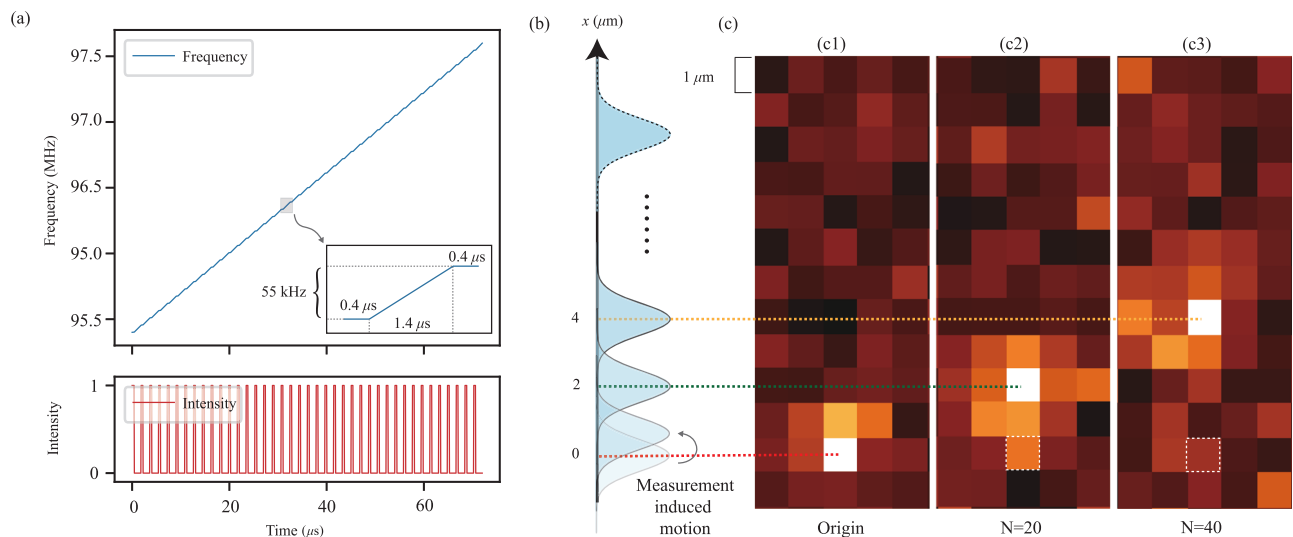
Fig. 5 | Controlled atomic motion via frequent measurements. a Measurement time sequence. The upper panel shows the frequency control sequence of the acousto-optic deflector (AOD) driving signal, with the frequency increasing stepwise from 95.4 MHz. The lower panel shows the intensity control sequence of the AOD driving signal, corresponding to the timing of the applied measurements. The measurement pulse width is 0.4 μs, with a 1.4 μs interval between measurements. The inset in the upper panel shows that the frequency variation of 55 kHz for every step occurs within the 1.4 μs interval when the intensity is zero. b Schematic of atomic wave packet motion. Each measurement pulse induces a slight shift in the
