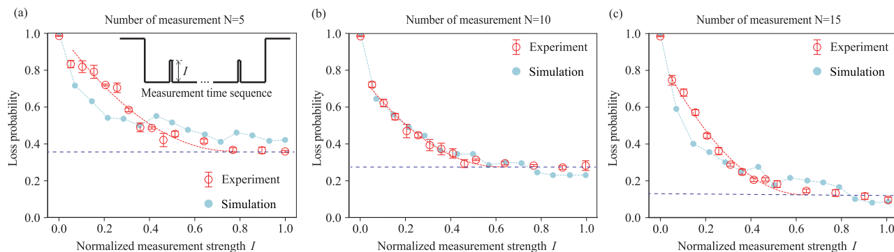
Fig. 3 | Evolution under different measurement strengths. During a 30 \mu\text{s} free evolution, N equally spaced measurement pulses of 0.4 \mu\text{s} duration are inserted. a–c show the final atom loss probability as a function of measurement strength for N = 5, 10, 15 , respectively. The experimental data are represented by red open circles, while the simulated results are indicated by light-blue filled circles. The inset in (a) displays measurement time sequence used in the experiment, where the level
