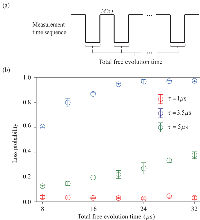
Fig. 4 | Free evolution interrupted by repeated measurements. a Experimental sequence. During free evolution, measurement pulses are inserted every 2 \mu\text{s} , with pulse widths set to 1 \mu\text{s} , 3.5 \mu\text{s} , and 5 \mu\text{s} , respectively. b Atom loss probability as a function of the total free evolution time for different pulse durations. For 1 \mu\text{s} pulses (red open circles), the loss probability remains negligible and independent of the evolution time. For 3.5 \mu\text{s} pulses (blue open circles), the loss probability increases rapidly with evolution time and approaches nearly unity beyond 24 \mu\text{s} . In contrast, for 5 \mu\text{s} pulses (green open circles), the loss probability rises much more slowly and stays below 0.4 even at 32 \mu\text{s} , indicating a substantial suppression of atom loss compared with the 3.5 \mu\text{s} case. The error bars represent the standard deviation.
