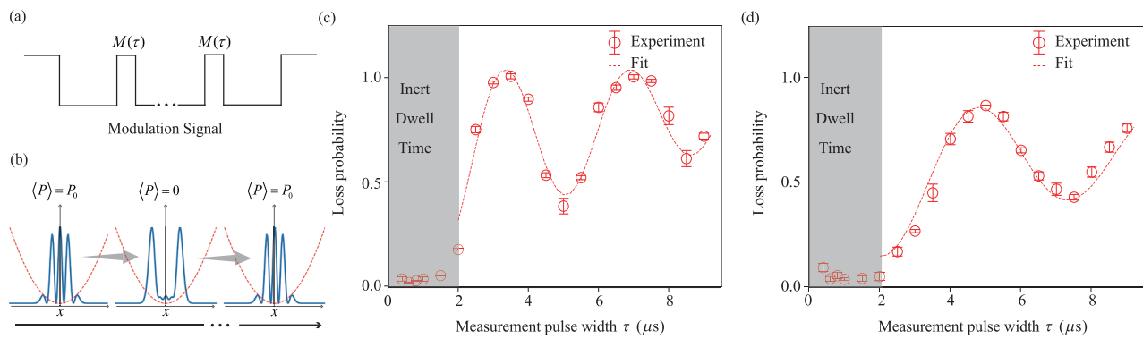
Fig. 2 | Dynamics of a single atom under finite-time measurements.
