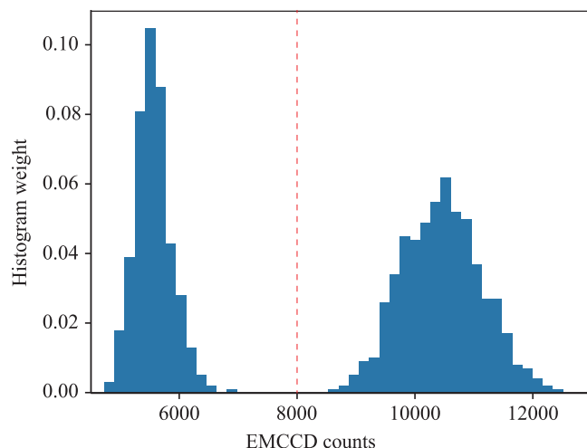
Fig. 6 | Histogram of single-atom fluorescence counts. The histogram shows the EMCCD count distribution from 1000 repeated fluorescence imaging experiments. The histogram exhibits a clear bimodal structure, with peaks centered at ~5500 and 10,500 counts, corresponding to empty traps and single-atom occupancy, respectively. The red dashed line denotes the threshold used to discriminate successful single-atom loading.
