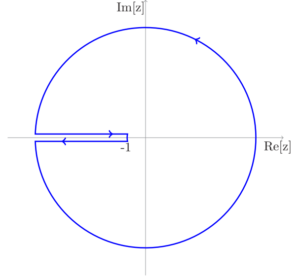
FIG. 5. Counterclockwise integration path C in Eq. (26) for evaluation of \phi_n for an unbounded lattice with the sampling rate \gamma\tau = \pi/2 . Equation (80) avoids the branch cut along the negative real axis when |z| > 1 . The outer radius approaches infinity.
