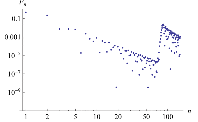
FIG. 11. Quantum walk on a ring with L = 100 sites for a sampling rate \gamma\tau = 0.6 with detection at the origin of the walk. For small n , the system exhibits a behavior similar to that of an infinite system (see Fig. 12). Roughly at n = 70 , there is a sudden increase in F_n , probably due to a partial revival of the packet at the origin.
