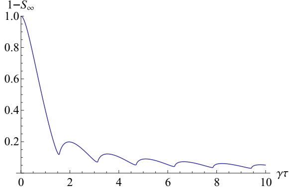
FIG. 10. For the one-dimensional tight-binding quantum walk, the probability that the particle is eventually detected 1 - S_\infty = \sum_{n=1}^{\infty} F_n versus the sampling rate \gamma\tau exhibits a nonmonotonic behavior. Unlike its classical random walk counterpart, the quantum walk is not recurrent, unless \gamma\tau \rightarrow 0 , which is the trivial case.
