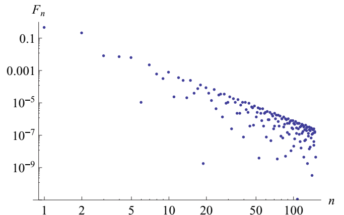
FIG. 12. Same as Fig. 11 for an infinite system.
