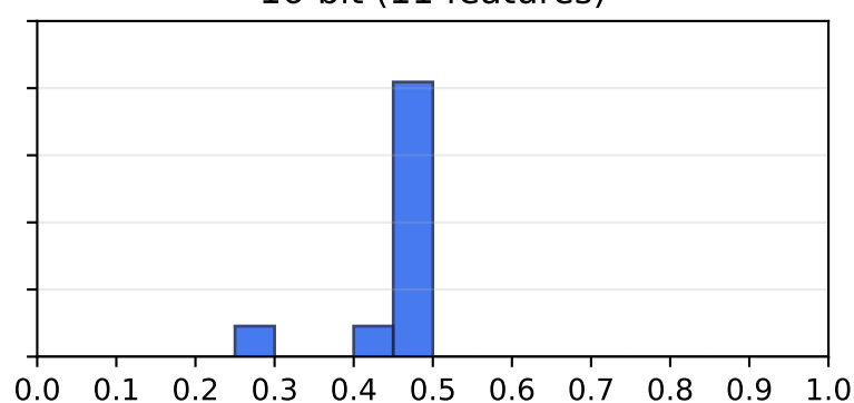
16-bit (11 features)
