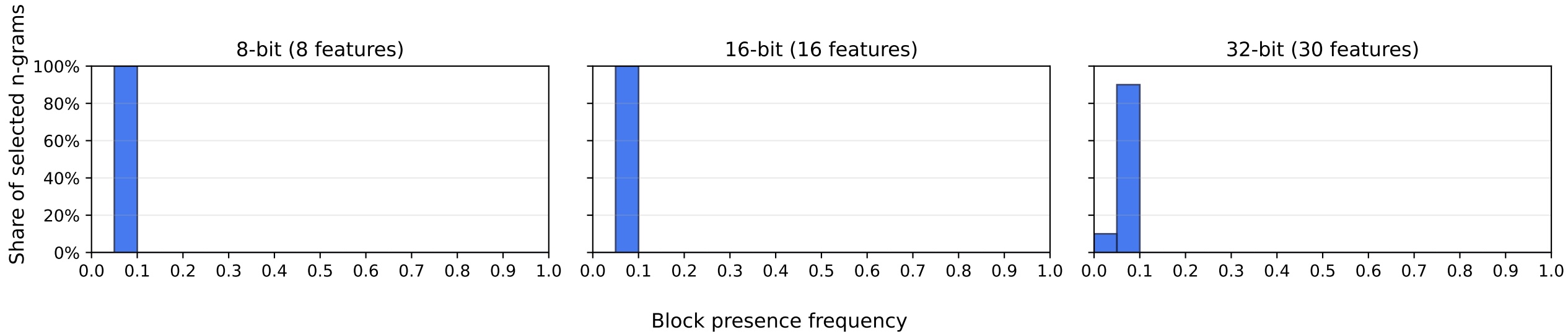
Selected n-gram block-frequency distributions fingerprint_distribution_entropy; n=2; frequency=[0.01, 0.1]
