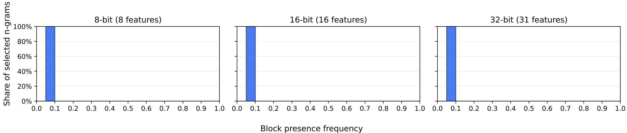
Selected n-gram block-frequency distributions fingerprint_distribution_entropy; n=2; frequency=[0.05, 0.1]
