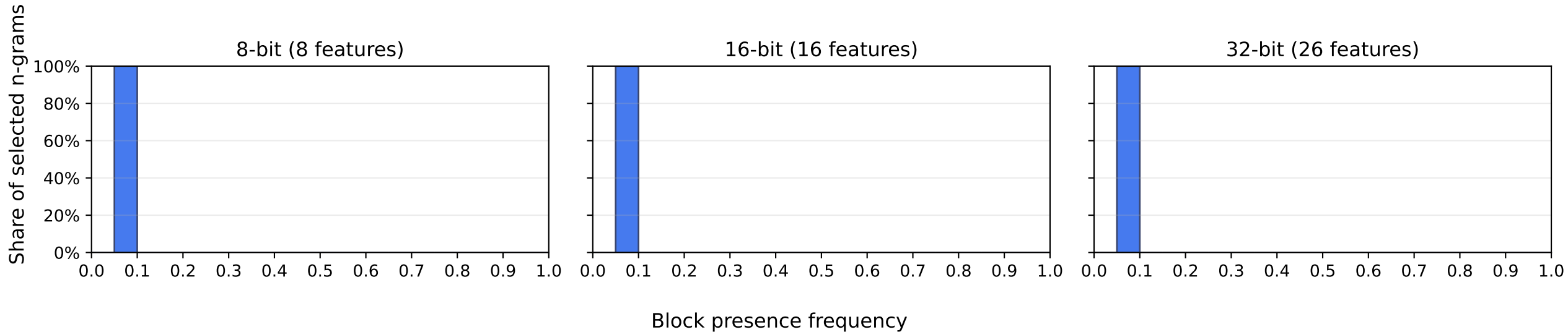
Selected n-gram block-frequency distributions fingerprint_distribution_entropy; n=3; frequency=[0.05, 0.1]
