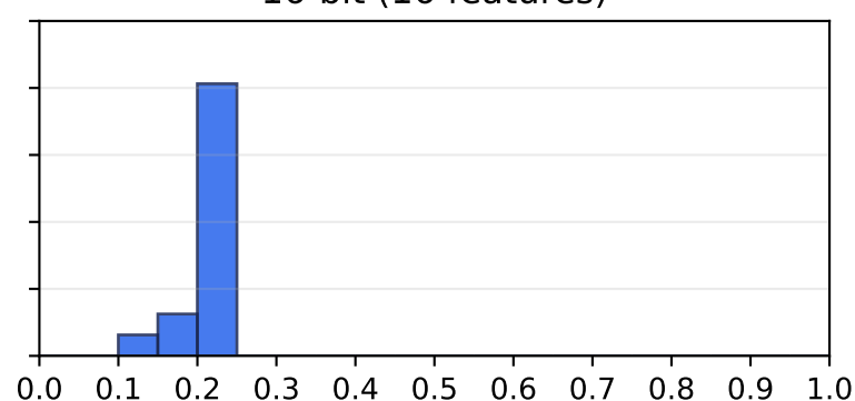
16-bit (16 features)
