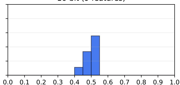
16-bit (9 features)
