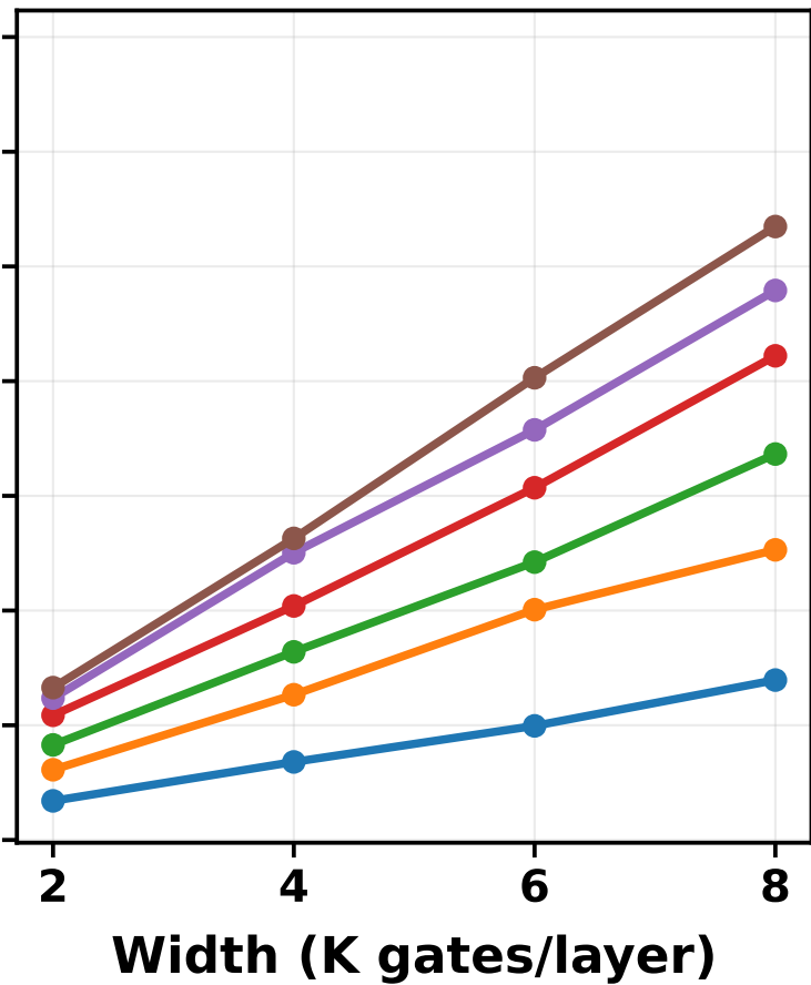
UCI Phishing
