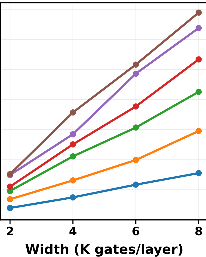
FashionMNIST
