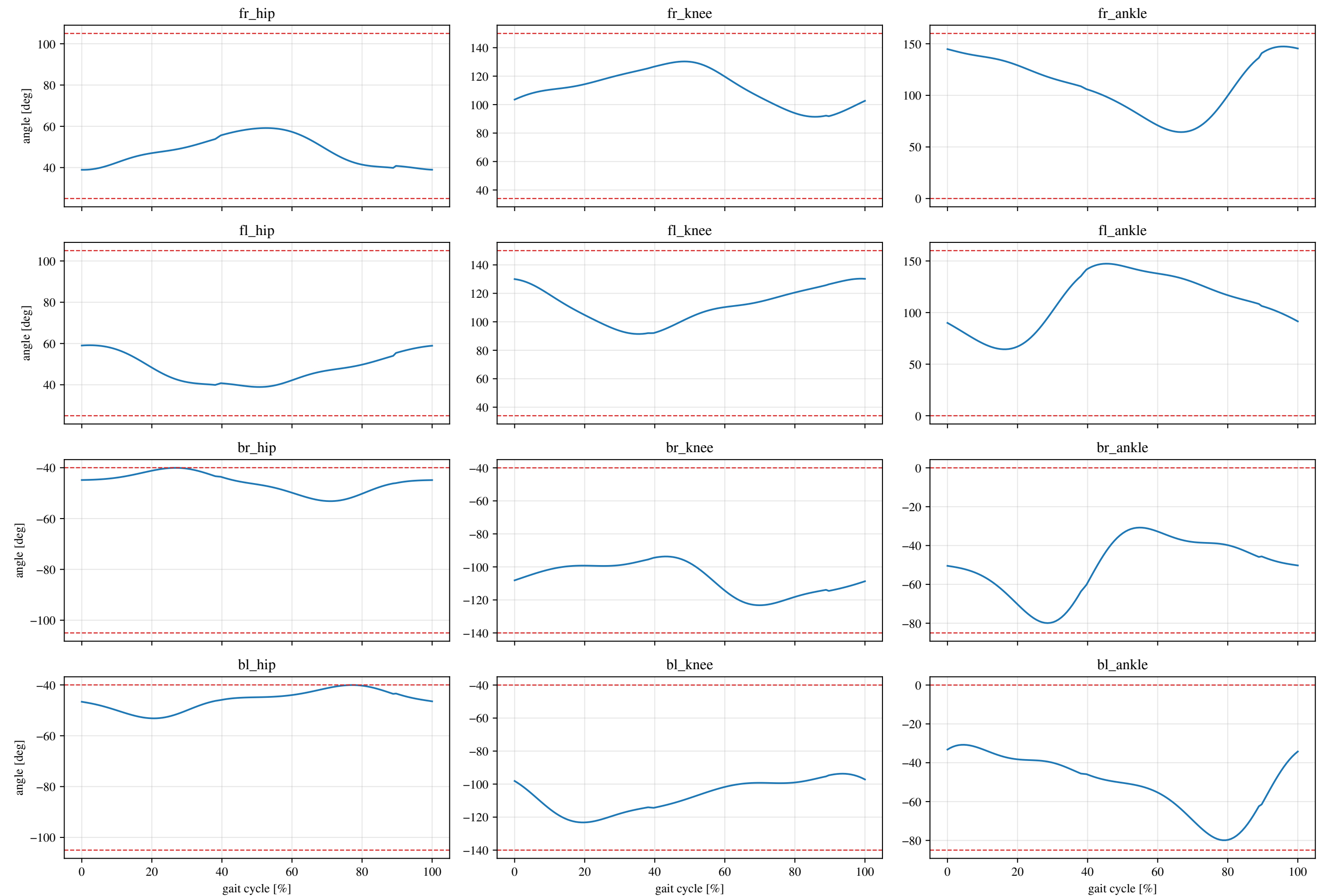
Joint angles — trajectory_adapted.npz (single gait cycle, 1 cycle = 127 frames (0.64 s))
