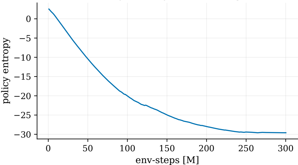
Policy entropy over training
