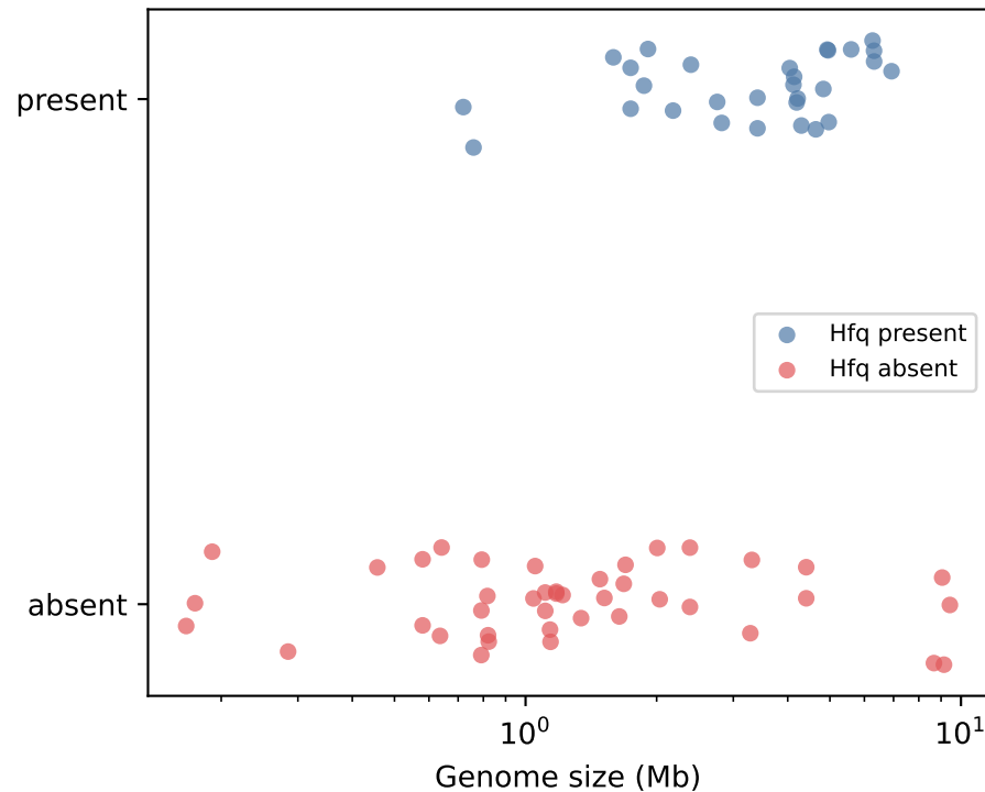
B Hfq presence vs genome size
