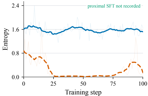
(b) Entropy
