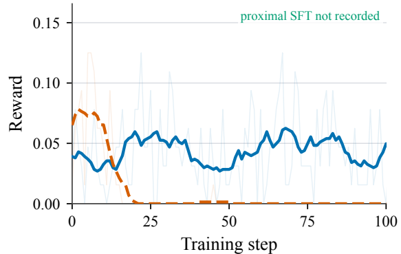
(c) Reward
