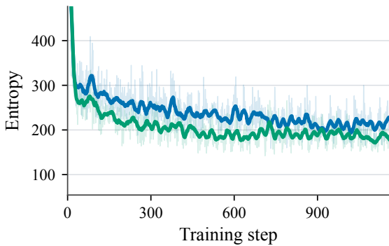
(a) Sequence entropy
