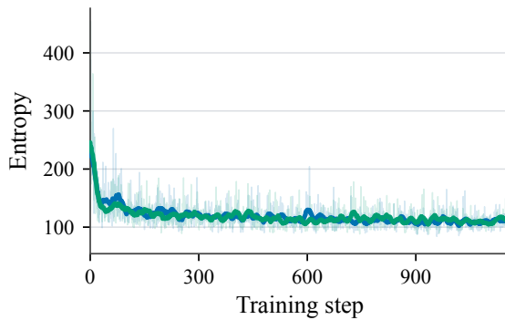
(b) True conditional entropy
