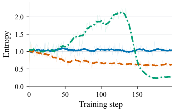
(c) Entropy
