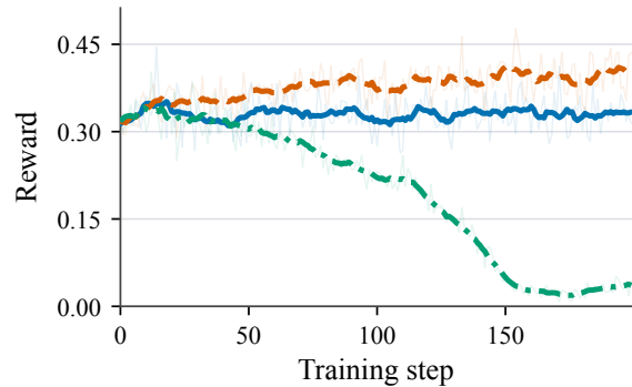
(b) Reward
