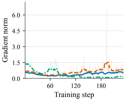
(a) Gradient norm
