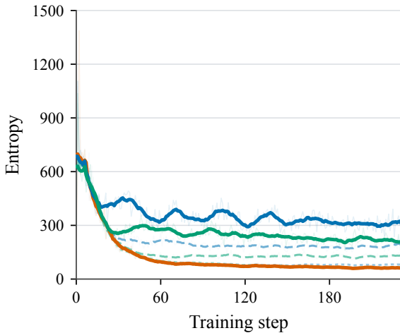
(a) Sequence entropy
