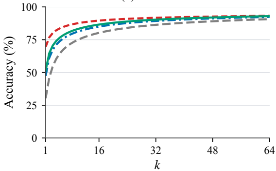
(a) MATH500
