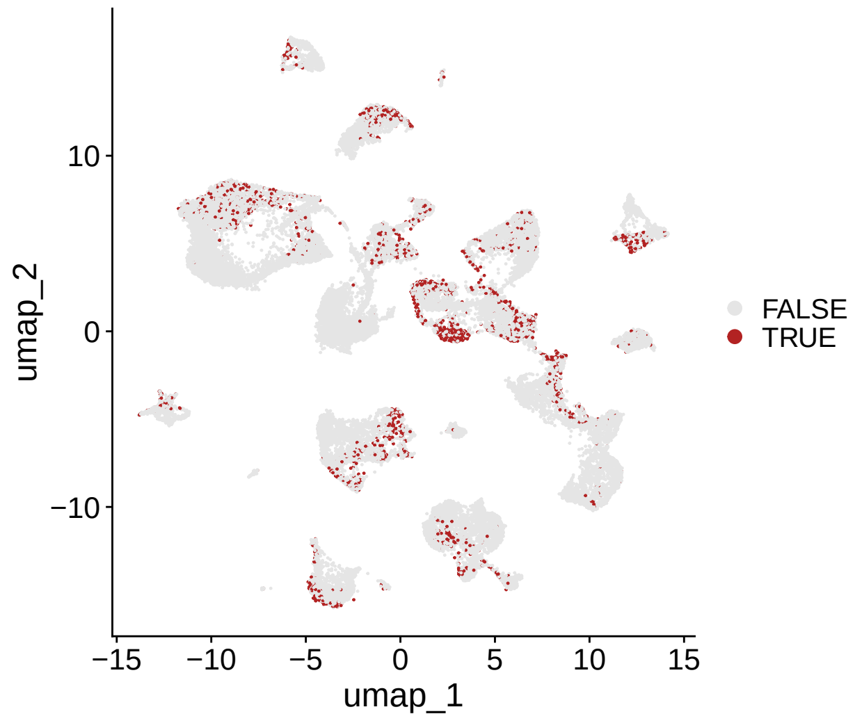
PROTEASOME_AUC_pos
