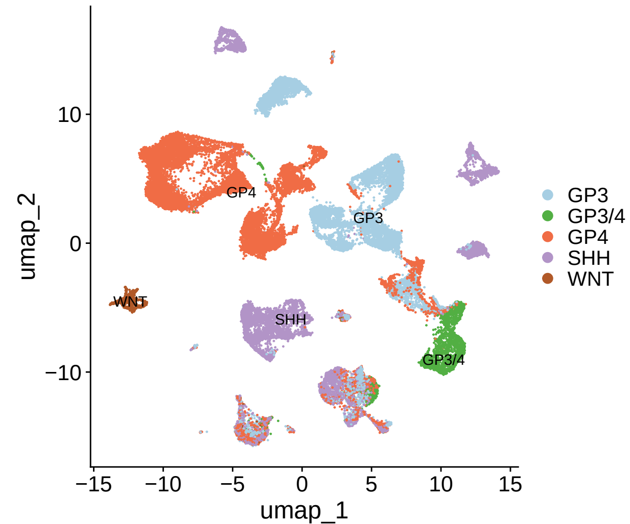
subgroup
