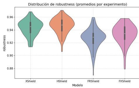
(c) Robustness
