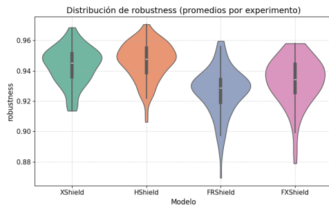
(c) Robustness
