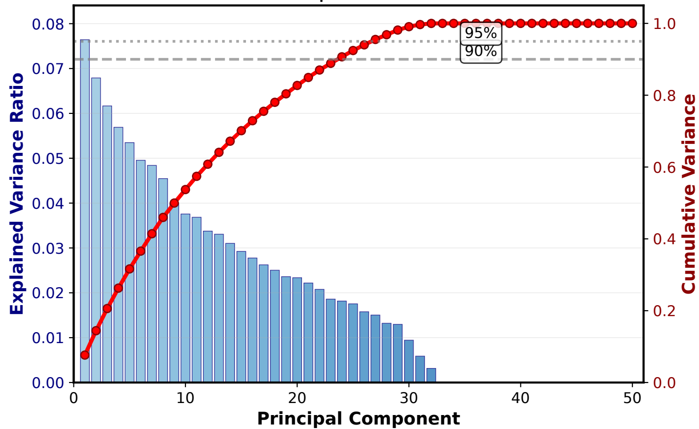
A. Effective Dimensionality 90% variance: 24 dims | 95% variance: 27 dims
