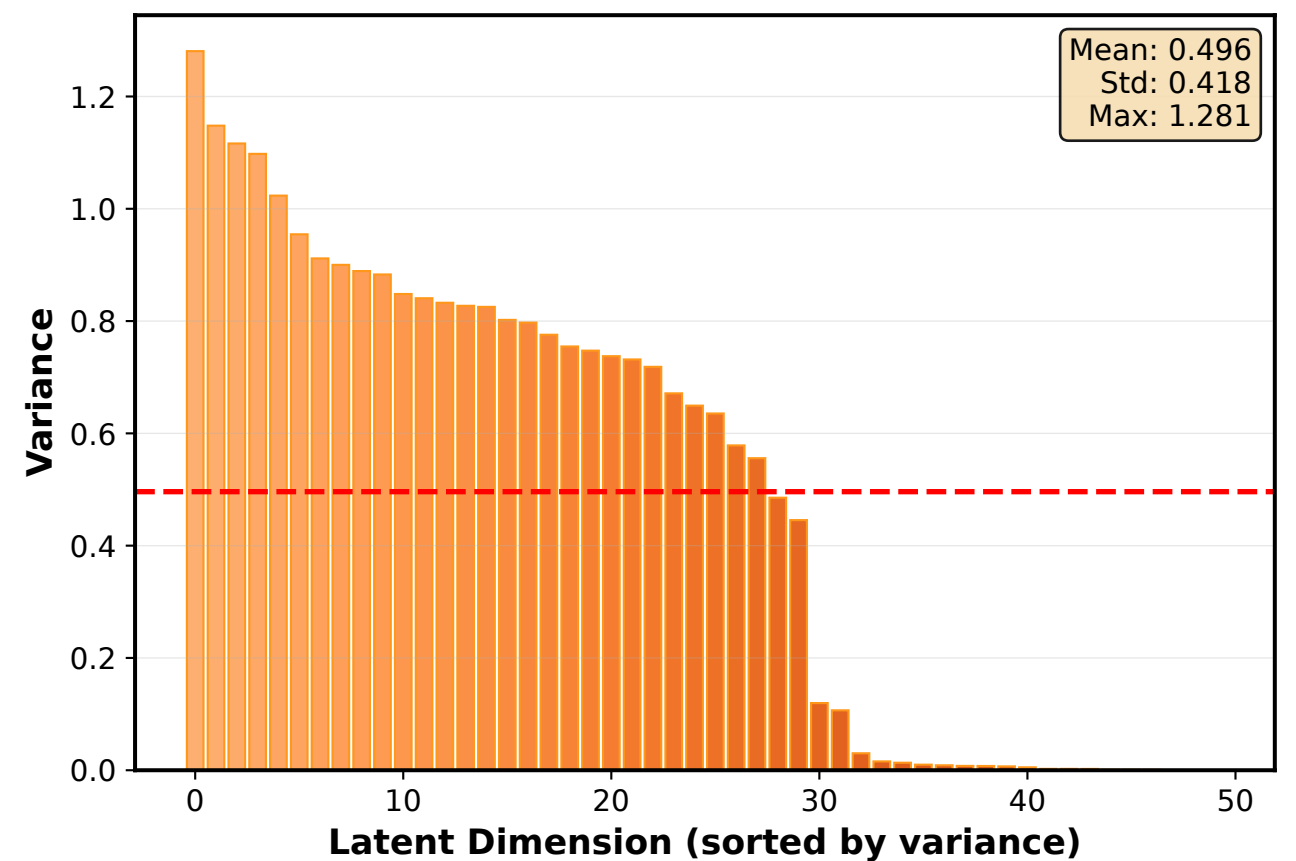
D. Latent Dimension Variance Distribution
