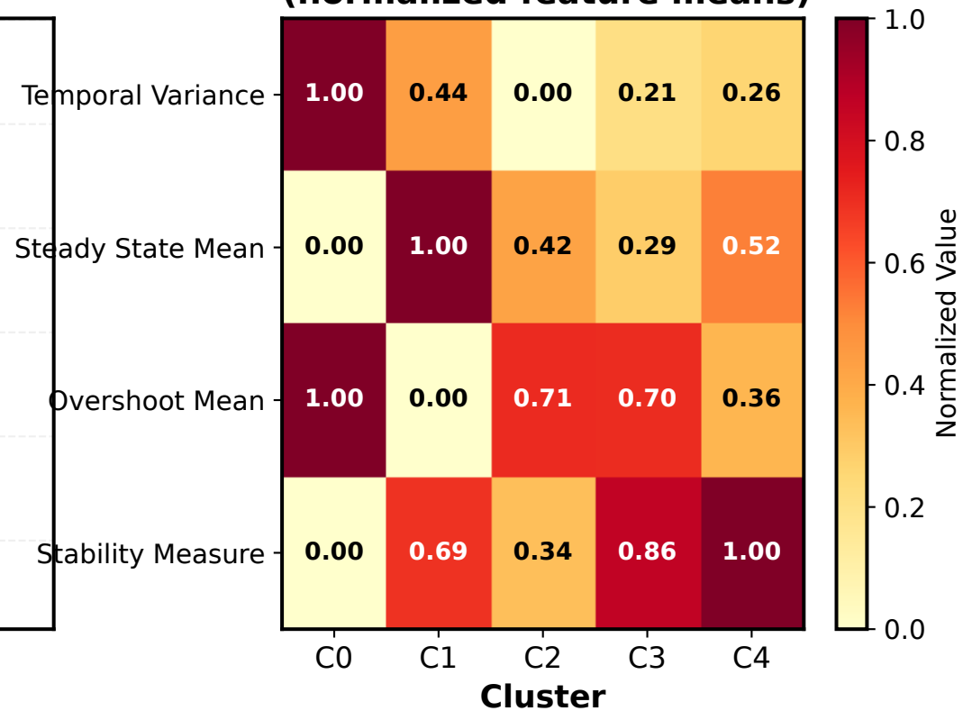
B. Cluster Characteristics (normalized feature means)
