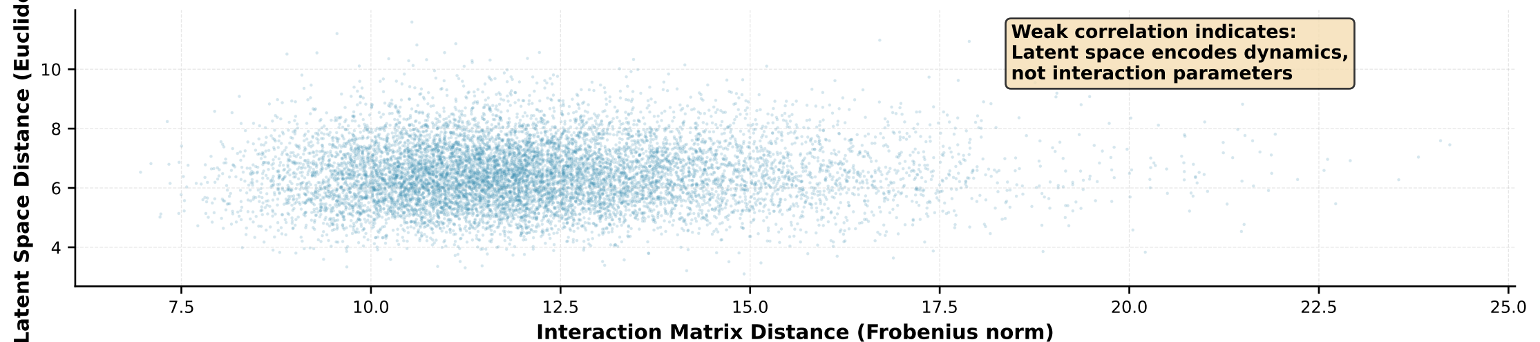
Distance Preservation: Interaction Matrices vs Latent Space Spearman \rho = 0.053 ( p = 2.13e-299 ) - No correlation
