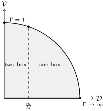
FIG. 5. Decision content and quantum content in the (\mathcal{D}, \mathcal{V}) plane at the symmetric preparation. Physical records lie in the quarter disk \mathcal{D}^2 + \mathcal{V}^2 \leq 1 (shaded, Eq. (37)). The coherent implementation traces the unit arc \mathcal{V} = \sqrt{1 - \mathcal{D}^2} , from \Gamma = 1 to the Omega point at (1, 0) , the ideal P-CTC limit; a dephased implementation lies on the \mathcal{V} = 0 axis (thick segment). The verdict of Eq. (19) reads only the horizontal coordinate: one-box for \mathcal{D} > m/M (dashed line drawn schematically; for M \gg m the true threshold m/M is close to \mathcal{D} = 0 and one-boxing occupies almost the whole axis, as in Fig. 4). The visibility is maximal at \Gamma = 1 and vanishes in the perfect-prediction limit.
