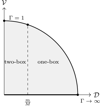
FIG. 4. Decision content and quantum content in the (\mathcal{D}, \mathcal{V}) plane at the symmetric preparation. Physical records lie in the quarter disk \mathcal{D}^2 + \mathcal{V}^2 \leq 1 (shaded, Eq. (37)). The coherent implementation traces the unit arc \mathcal{V} = \sqrt{1 - \mathcal{D}^2} , from \Gamma = 1 to the ideal P-CTC limit; a dephased implementation lies on the \mathcal{V} = 0 axis (thick segment). The verdict of Eq. (19) reads only the horizontal coordinate: one-box for \mathcal{D} > m/M (dashed line drawn schematically; for M \gg m the true threshold m/M is close to \mathcal{D} = 0 and one-boxing occupies almost the whole axis, as in Fig. 3). The visibility is maximal at \Gamma = 1 and vanishes in the perfect-prediction limit.
