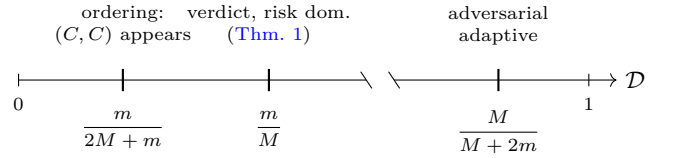
FIG. 3. The threshold ladder on the distinguishability axis \mathcal{D} = (\Gamma - 1)/(\Gamma + 1) ; positions are schematic. The one-boxing equilibrium appears at \mathcal{D} = m/(2M + m) , the convention-independent verdict and risk dominance switch at \mathcal{D} = m/M , and a nonzero one-boxing Born weight survives the adversarial adaptive prior only above \mathcal{D} = M/(M + 2m) (Sec. VI). For Gardner’s values M = \$1,000,000 and m = \$1,000 the three thresholds sit at \mathcal{D} \approx 5.0 \times 10^{-4} , \mathcal{D} = 10^{-3} , and \mathcal{D} \approx 0.998 : the game-structure and verdict thresholds lie within 10^{-3} of \mathcal{D} = 0 and the adversarial threshold within 2 \times 10^{-3} of \mathcal{D} = 1 .
