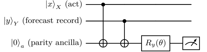
FIG. 2. Forward-time opening of the Bell contraction. The CNOT gates write the record parity x \oplus y into the ancilla; after R_y(\theta) , the branch is retained only for the outcome a = 0 . Agreement and mismatch then survive with weights \cos^2(\theta/2) and \sin^2(\theta/2) , and the retained Kraus operator is exactly K(\theta) = C_{\mathcal{U}_\theta} .
