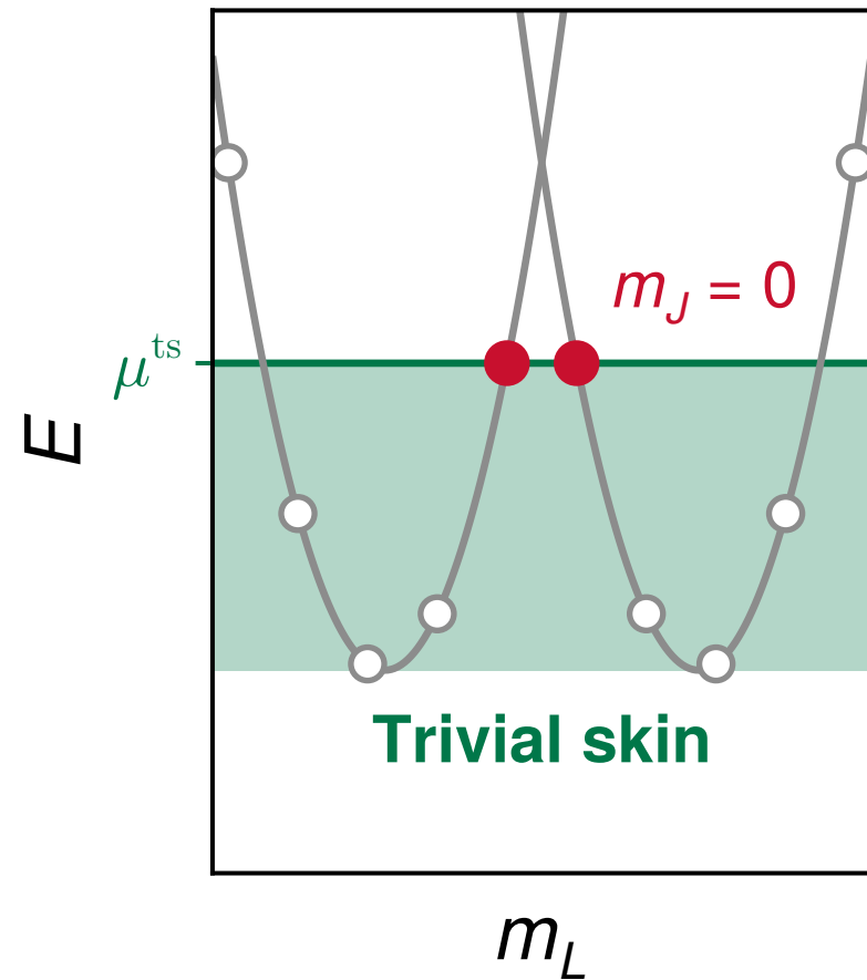
m_J = 0 threshold
