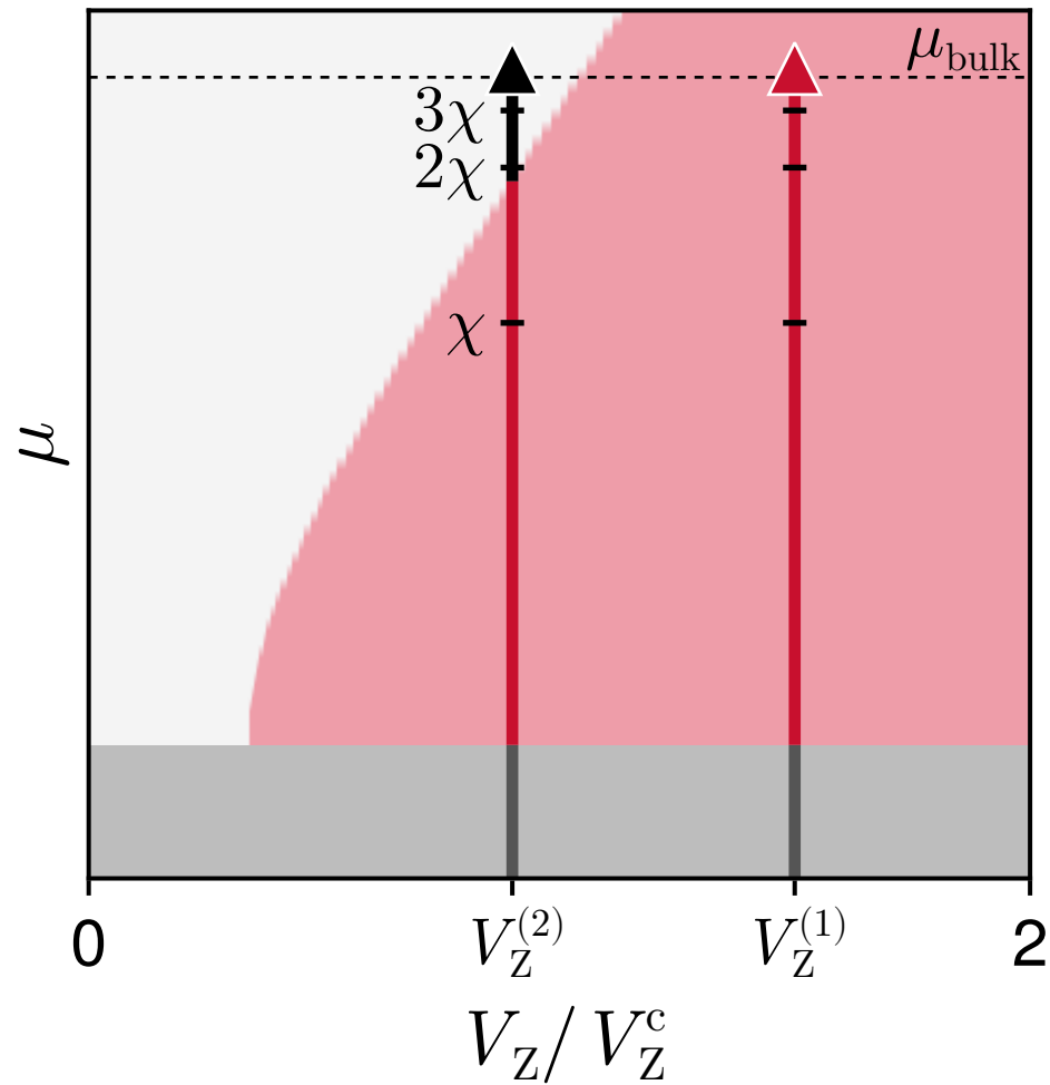
Partial shell
