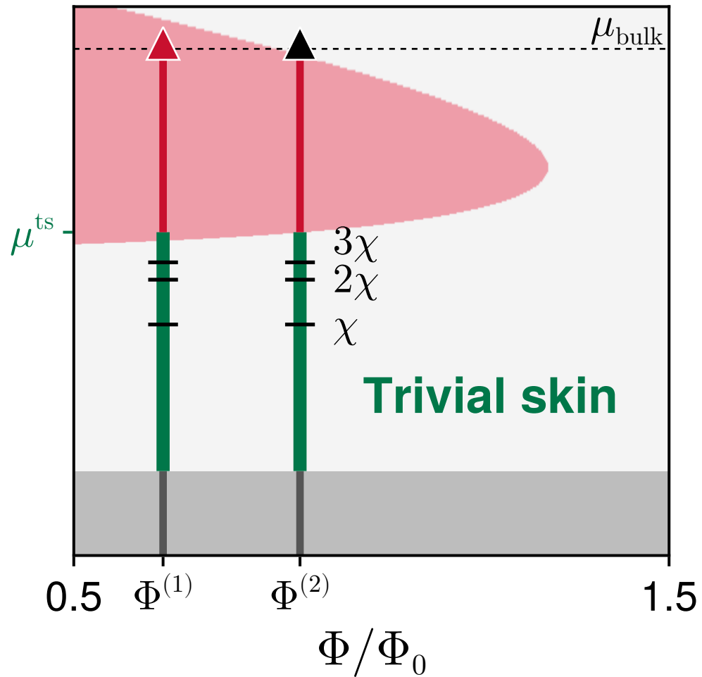
Full shell
