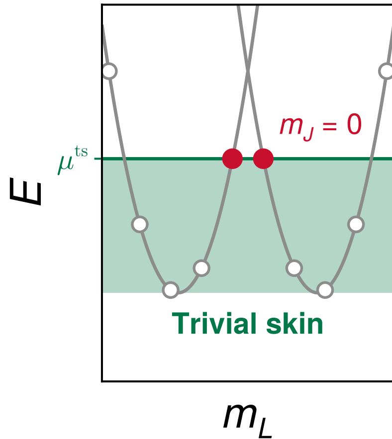
m_J = 0 threshold
