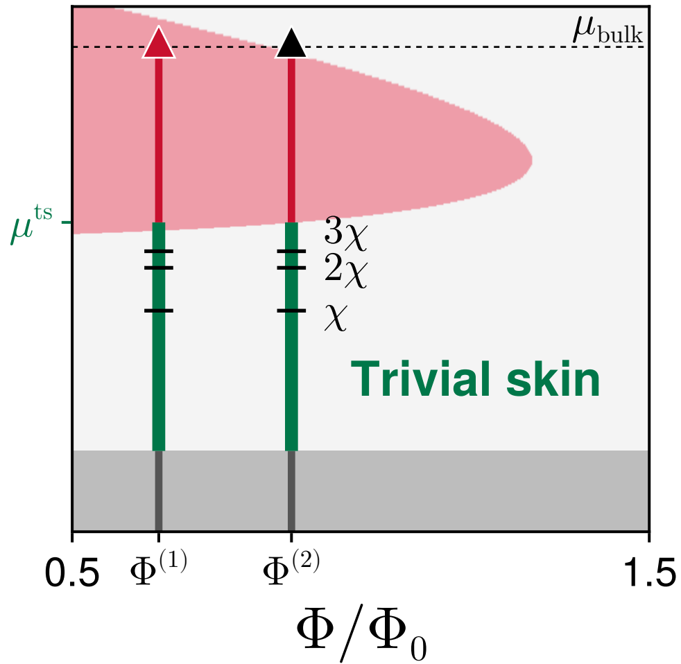
Full shell
