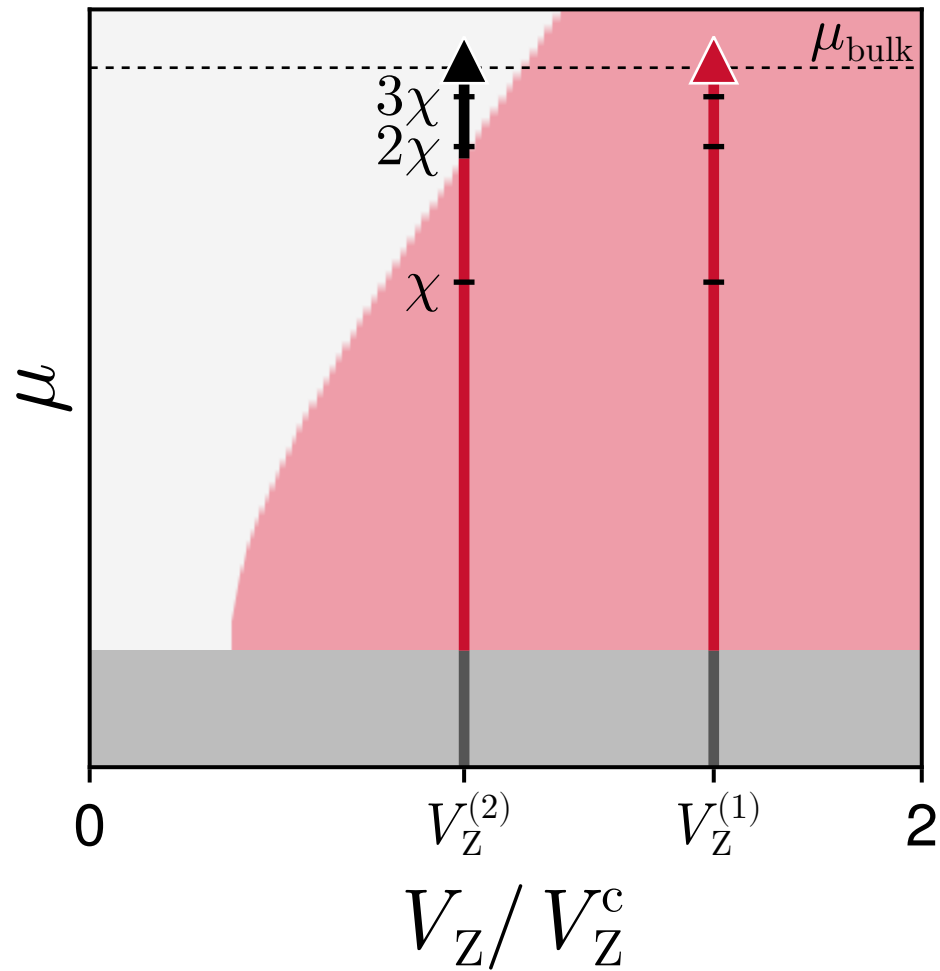
Partial shell
