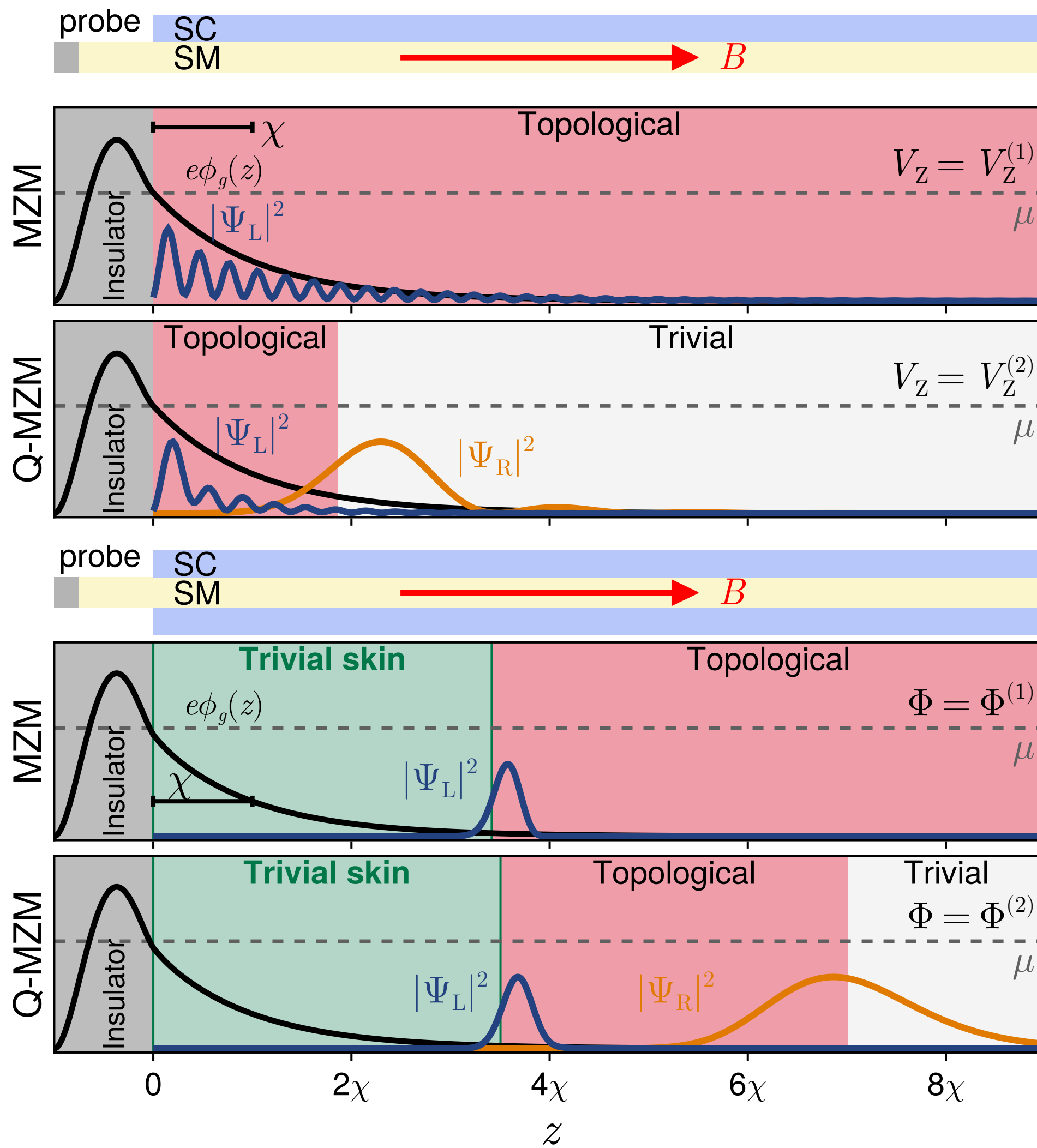
Real space
