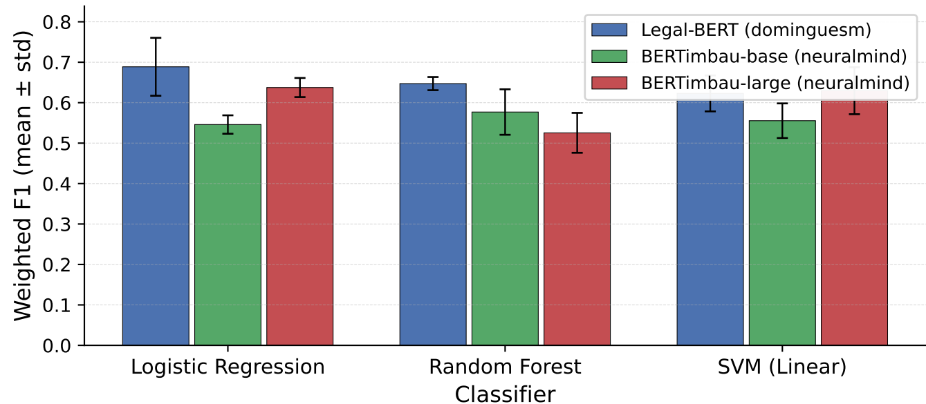
Stage 2 encoder comparison by downstream classifier
