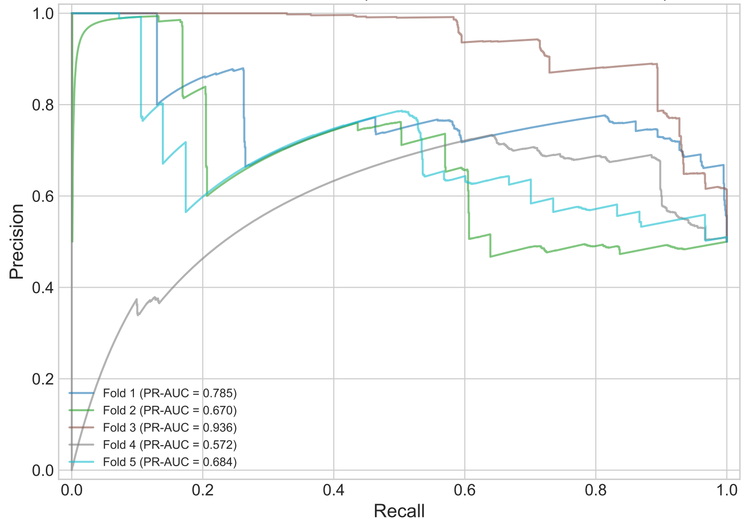
Precision-Recall Curves (Mean PR-AUC = 0.729 \pm 0.124 )
