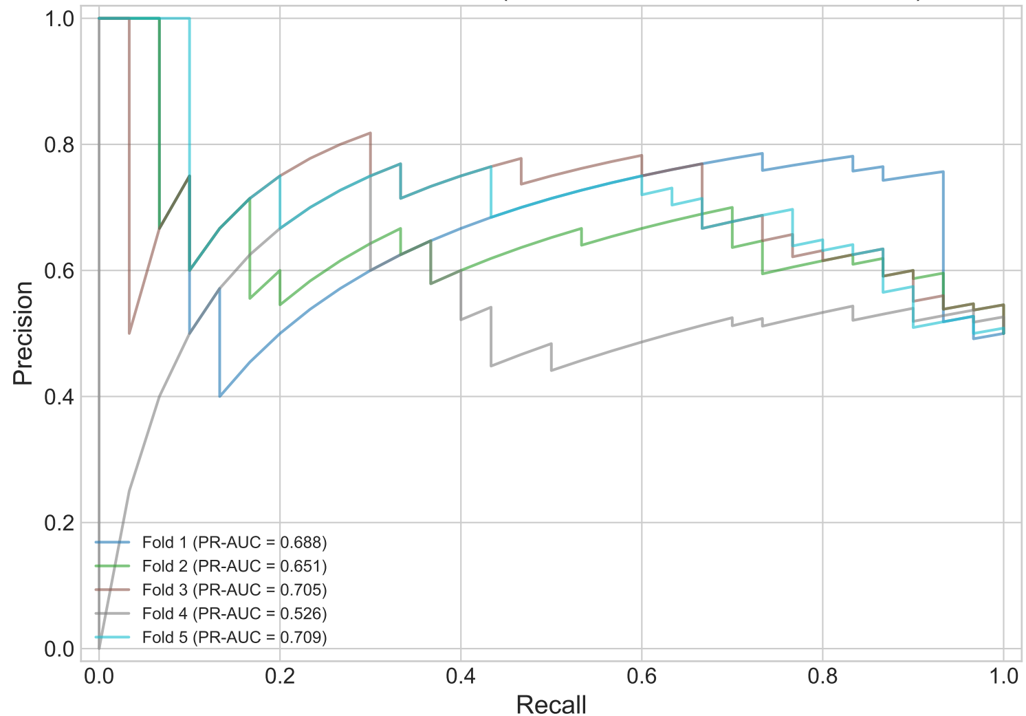
Precision-Recall Curves (Mean PR-AUC = 0.656 \pm 0.068 )
