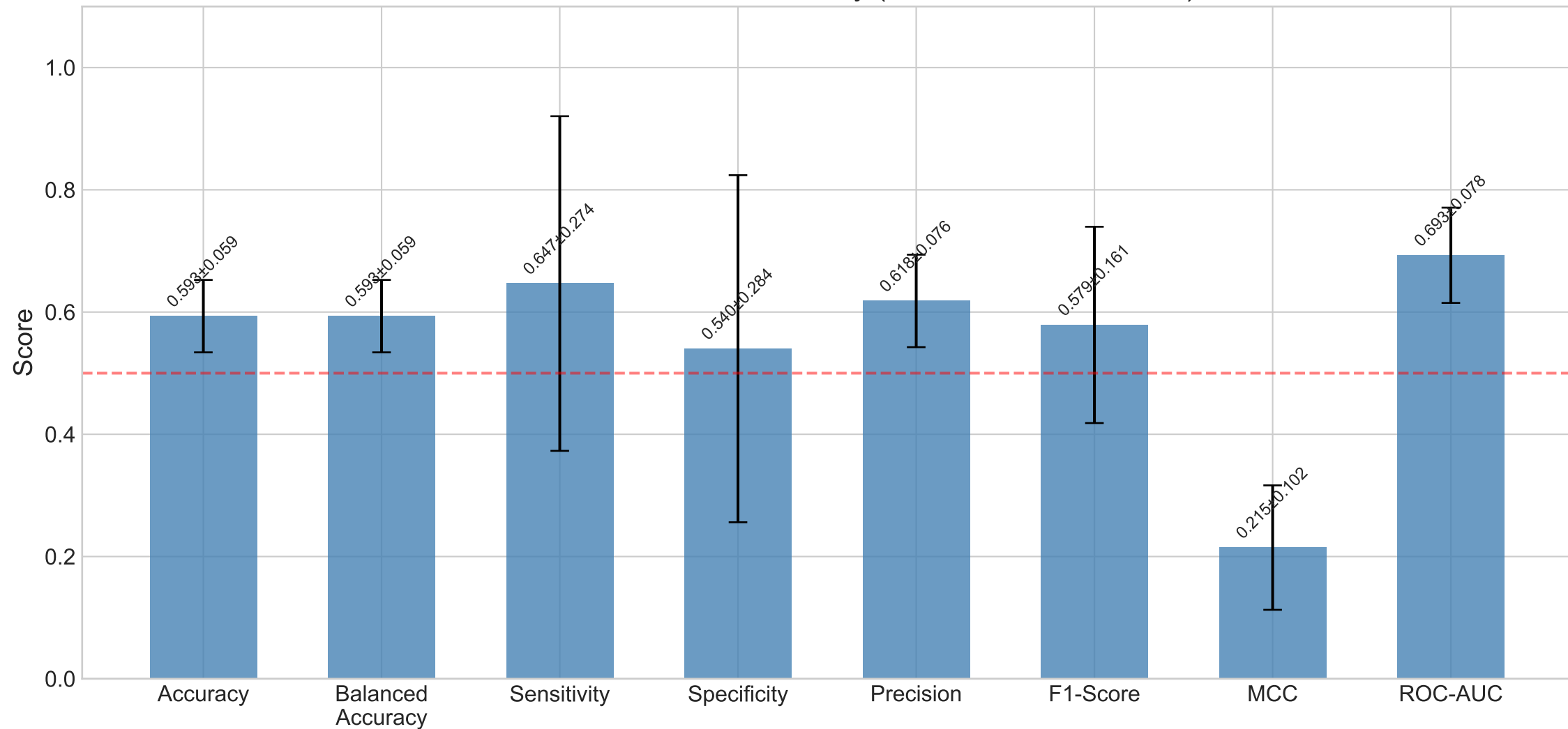
Performance Metrics Summary (5-Fold CV, Mean \pm Std)
