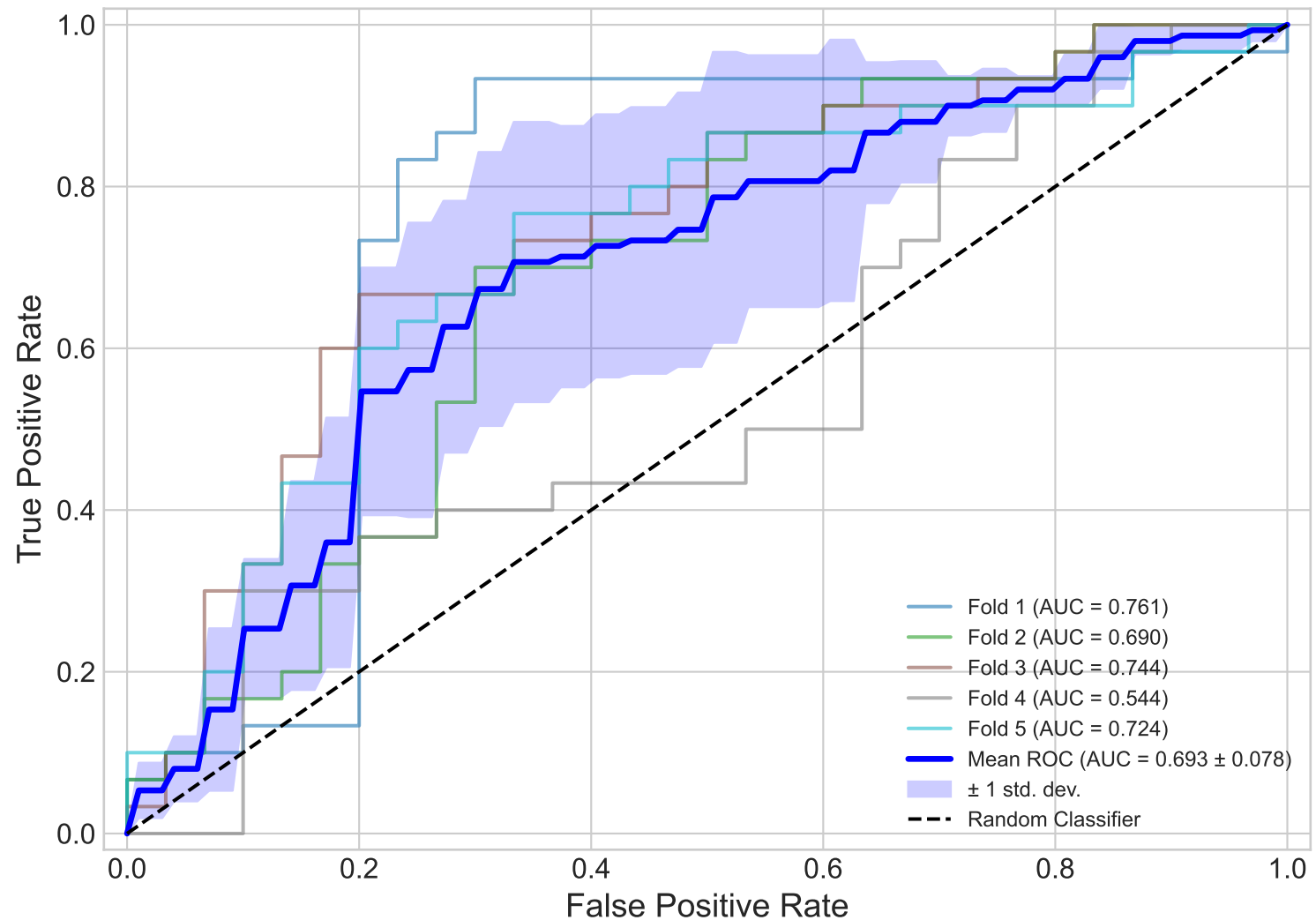
ROC Curves - 5-Fold Cross-Validation
