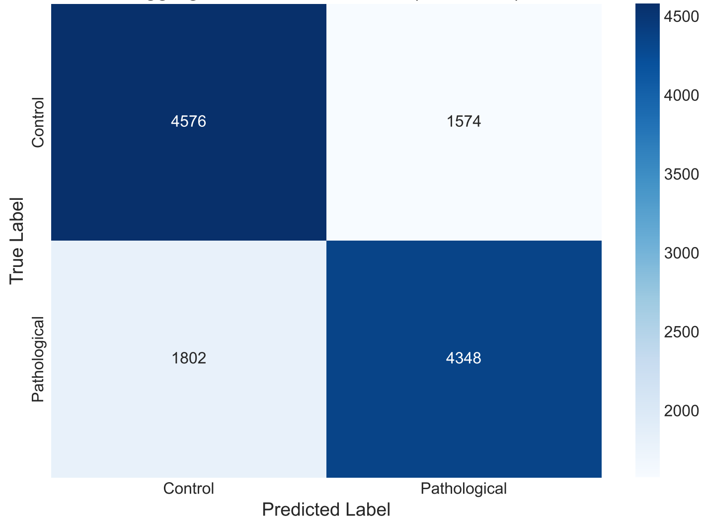
Aggregated Confusion Matrix (5-Fold CV)
