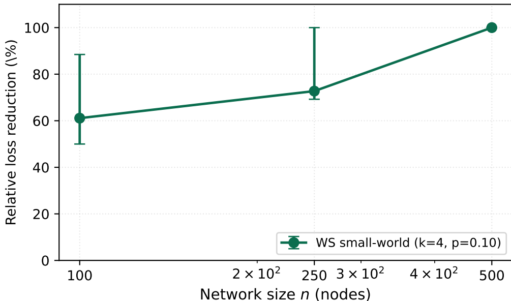
EMMET-DP scaling on WS small-world (100 seeds/config)
