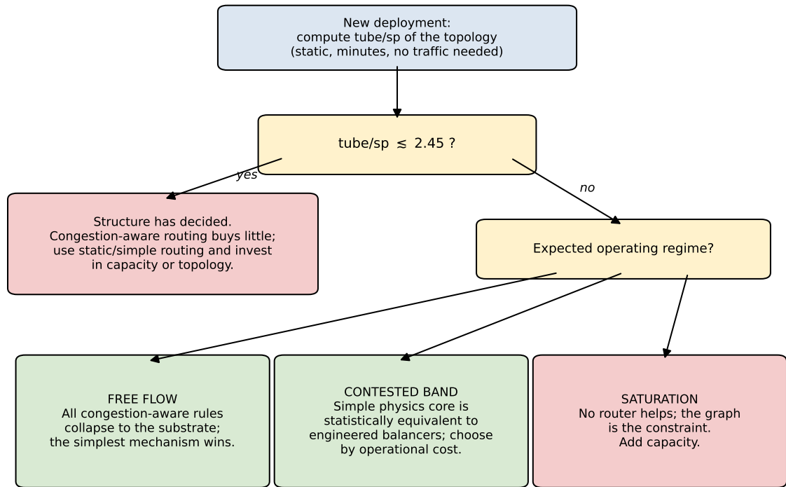
Figure 3: The two-factor law as a pre-deployment decision diagram. The structural ratio tube/sp is computable from topology alone, before any traffic exists; the break-even \approx 2.45 and the regime boundaries are the bench estimates of Sections 10 and 12.5.
