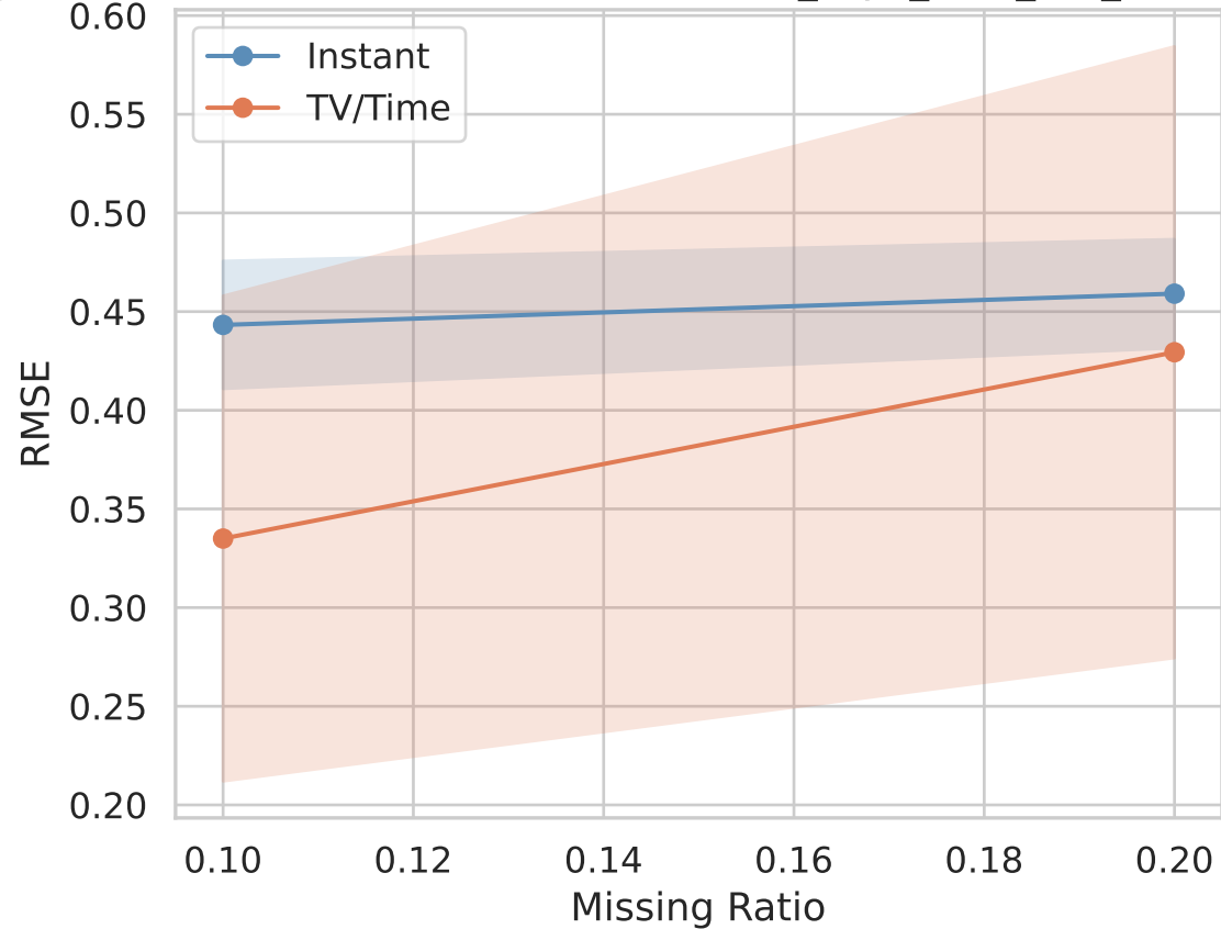
RMSE — TV/Time vs Instant — it36_3syn_beta_low_missing
