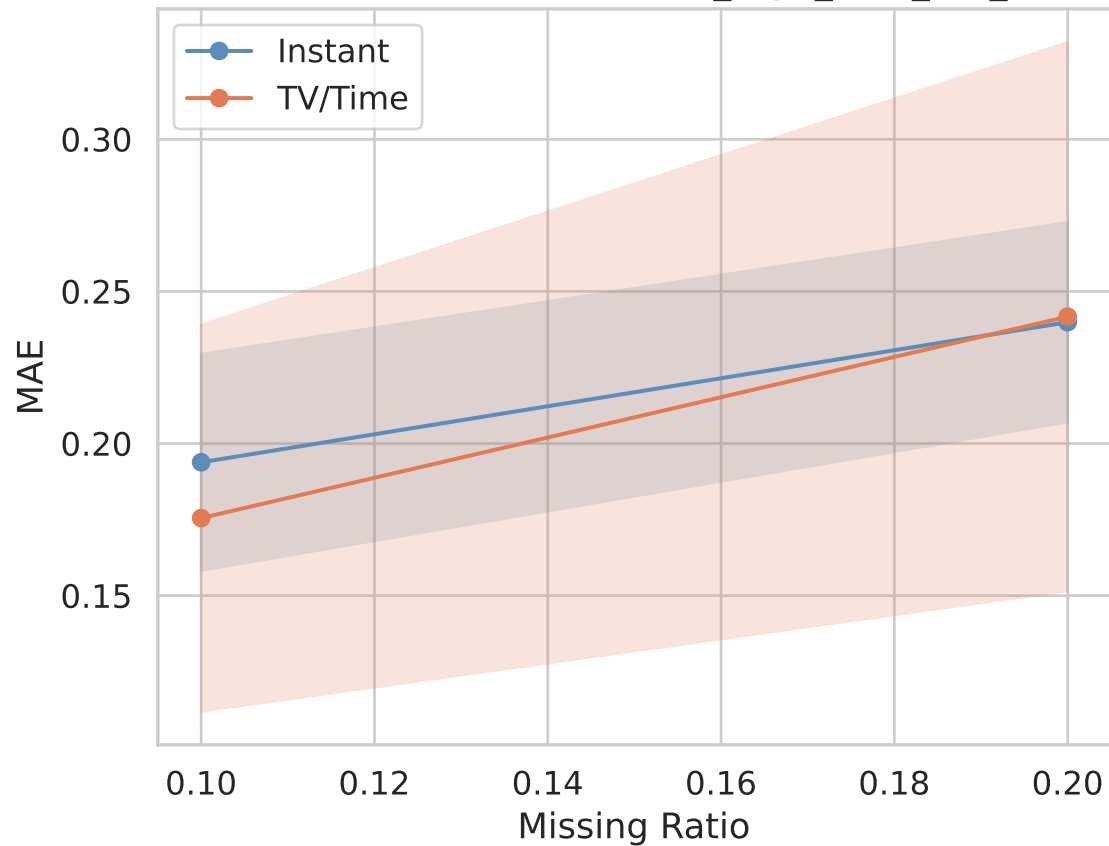
MAE — TV/Time vs Instant — it36_3syn_beta_low_missing
