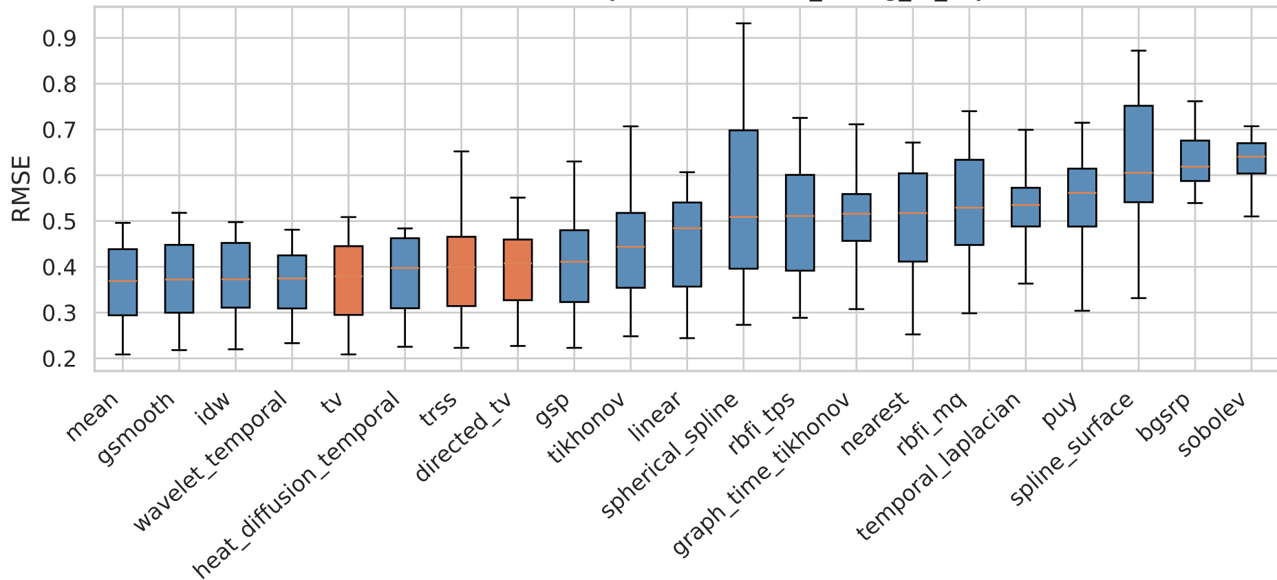
RMSE Distribution by Method — it31_strong_tv_3syn
