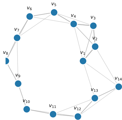
(a) Grafo de electrodos \mathcal{G} = (\mathcal{V}, \mathcal{E}, \mathbf{W})
