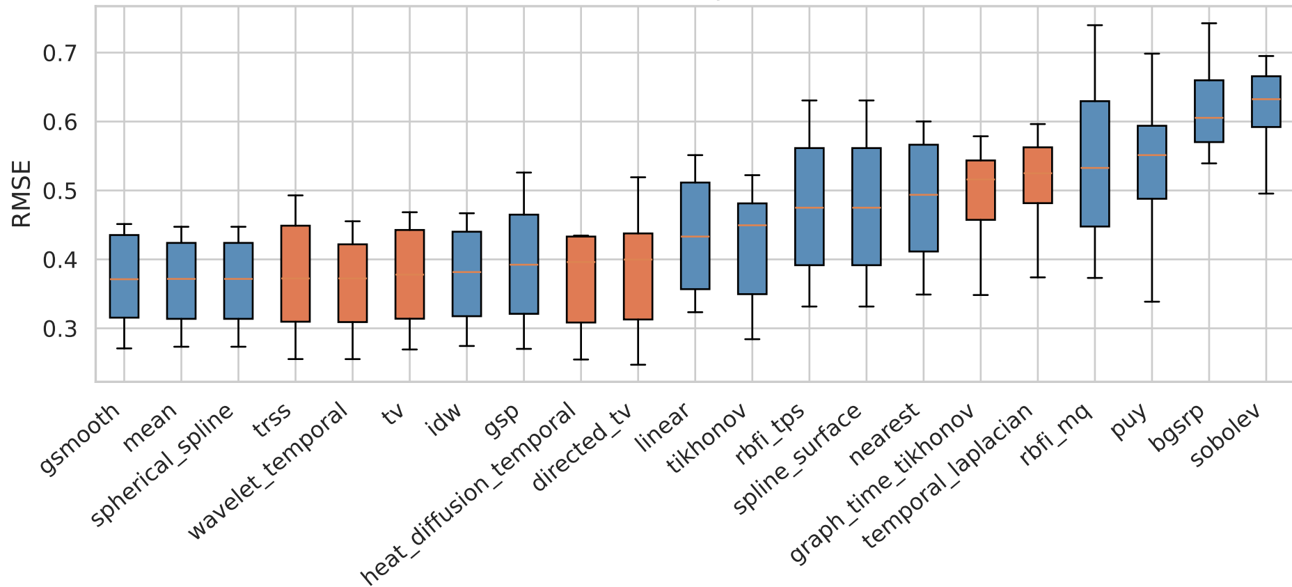
RMSE Distribution by Method — it02
