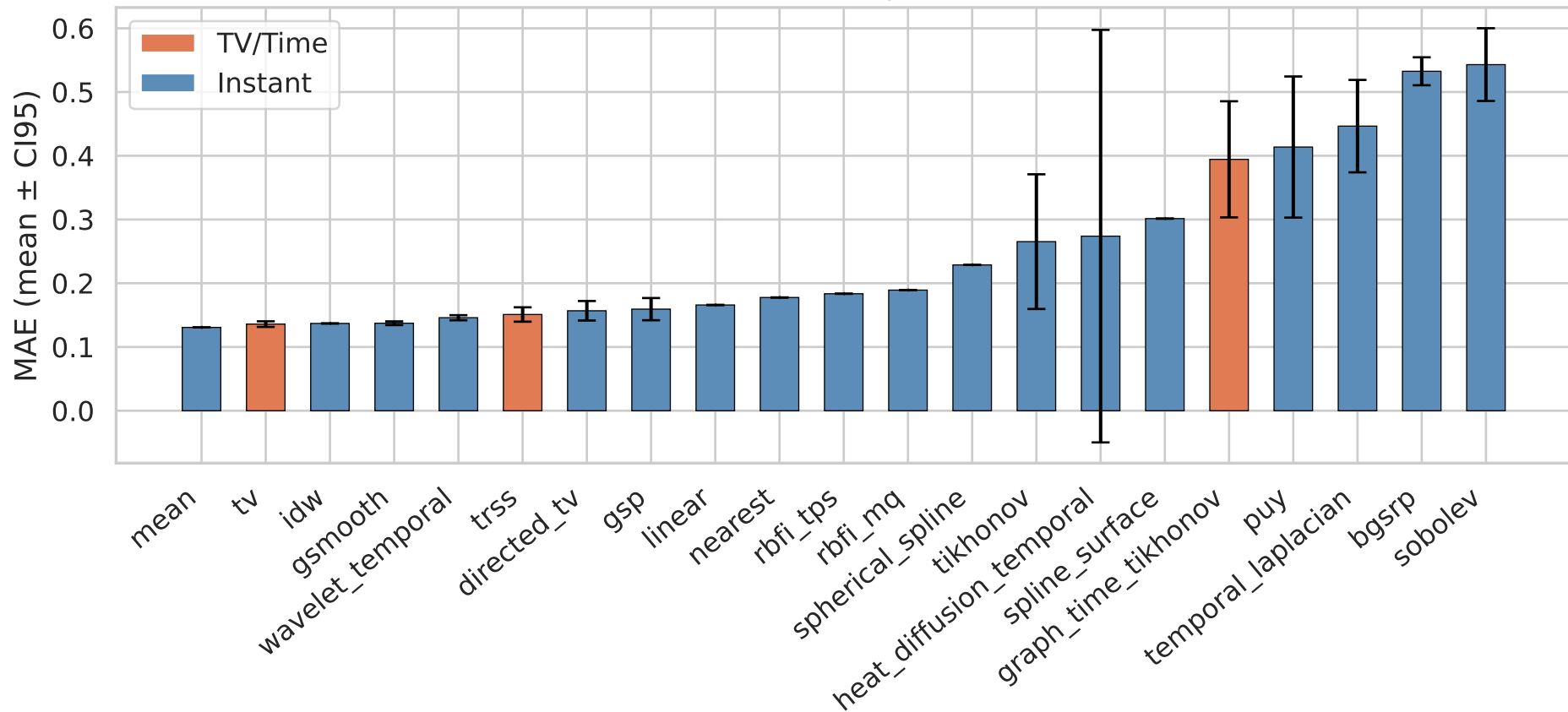
Mean Absolute Error by Method — it01
