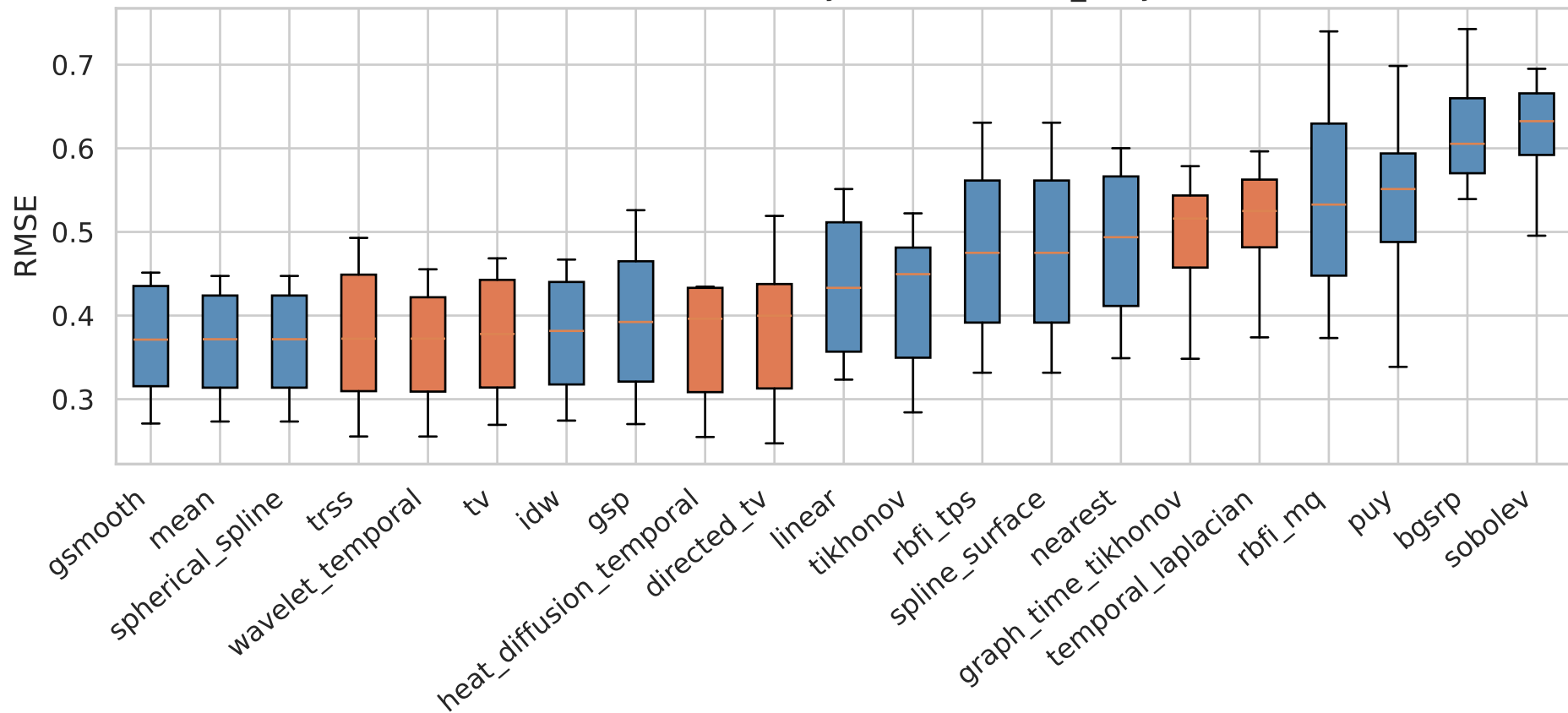
RMSE Distribution by Method — it01_retry
