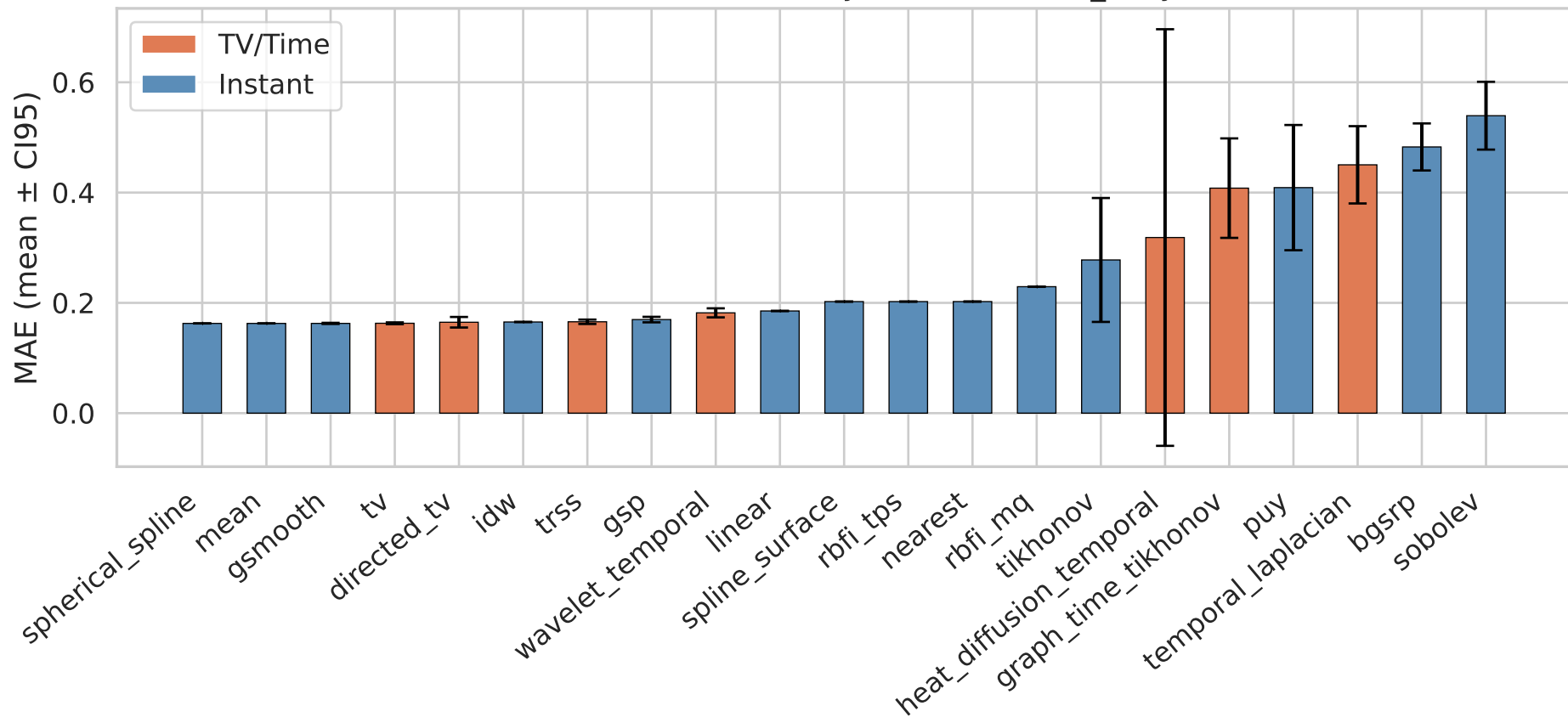
Mean Absolute Error by Method — it01_retry
