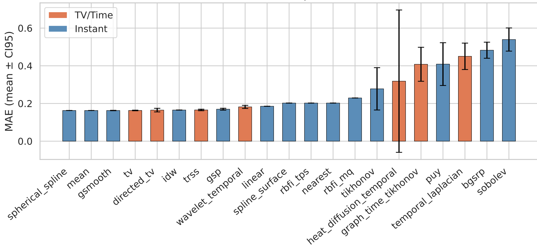
Mean Absolute Error by Method — it02
